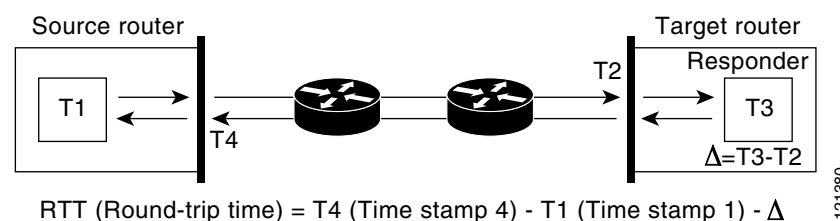
Figure 58-2 Cisco IOS IP SLAs Responder Time Stamping
