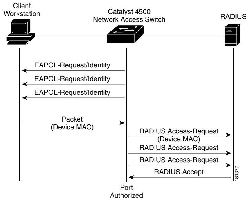
Figure 40-6 Message Exchange during MAC Authentication Bypass
