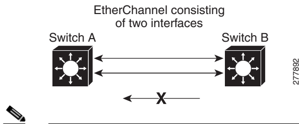
Figure 28-2 Fast UDLD Topology
