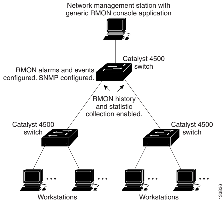
Figure 59-1 Remote Monitoring Example
