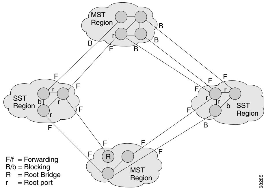
Figure 18-2 Network with Interconnected SST and MST Regions
