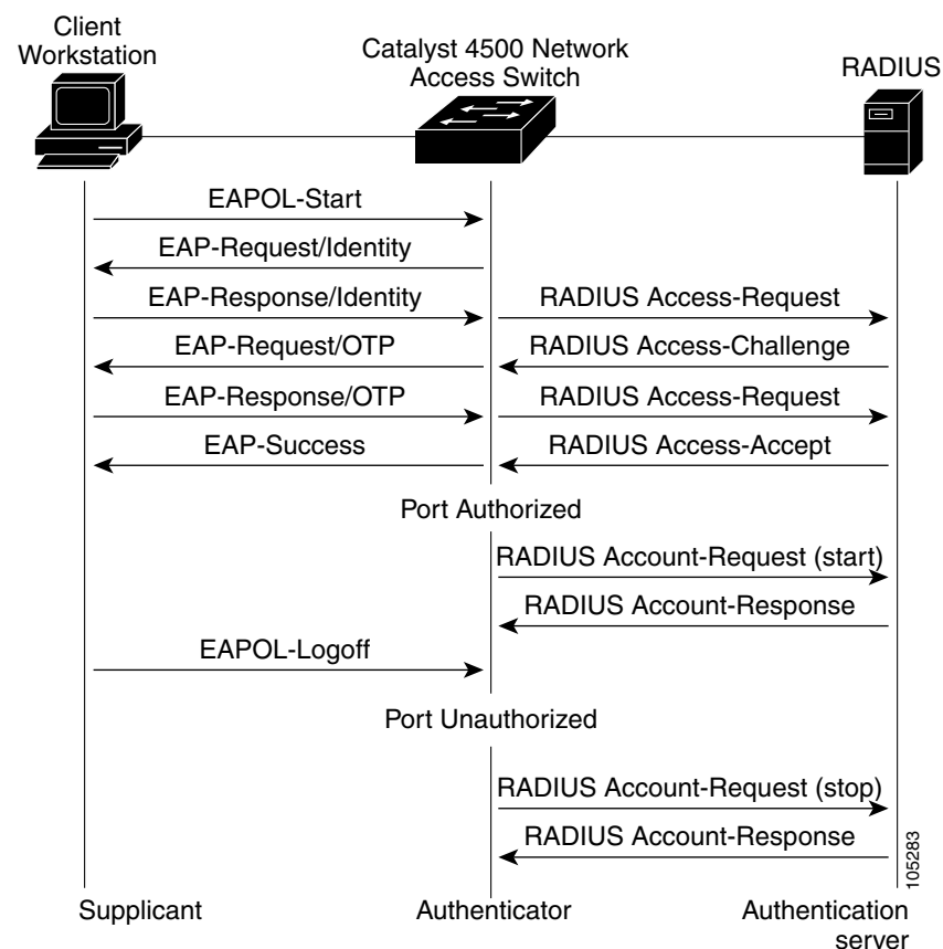
Figure 32-5 RADIUS Accounting
