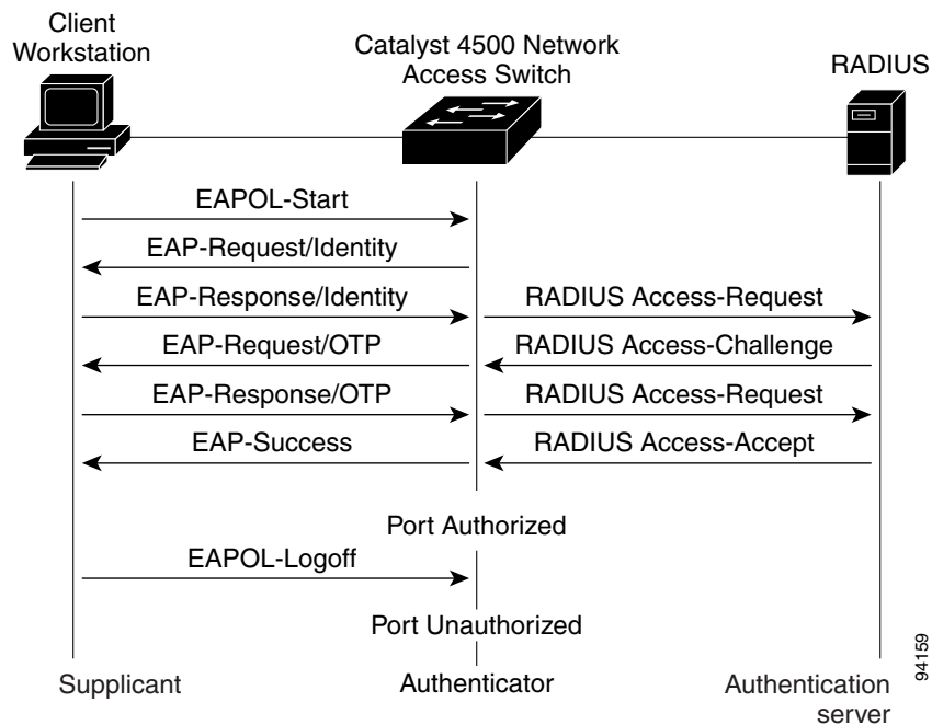
Figure 32-2 Message Exchange
