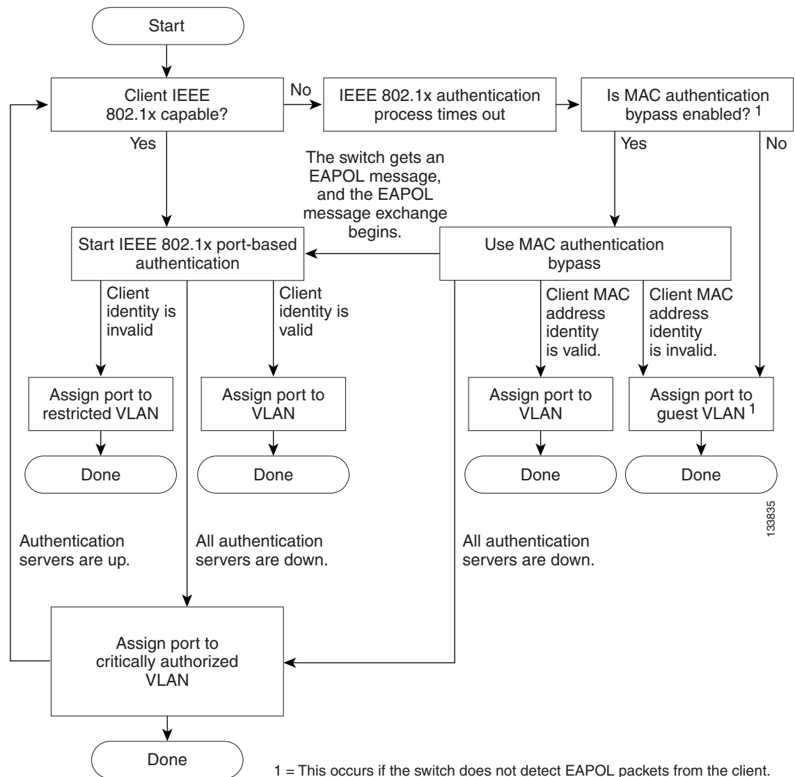
Figure 32-3 Authentication Flowchart
