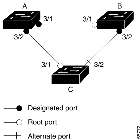
Figure 18-1 Triangular Switch Configuration with Loop Guard
