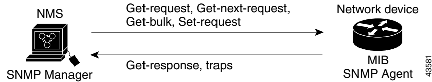
Figure 43-1 SNMP Network
