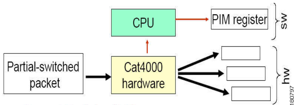
Figure 49-6 Partial Switching
