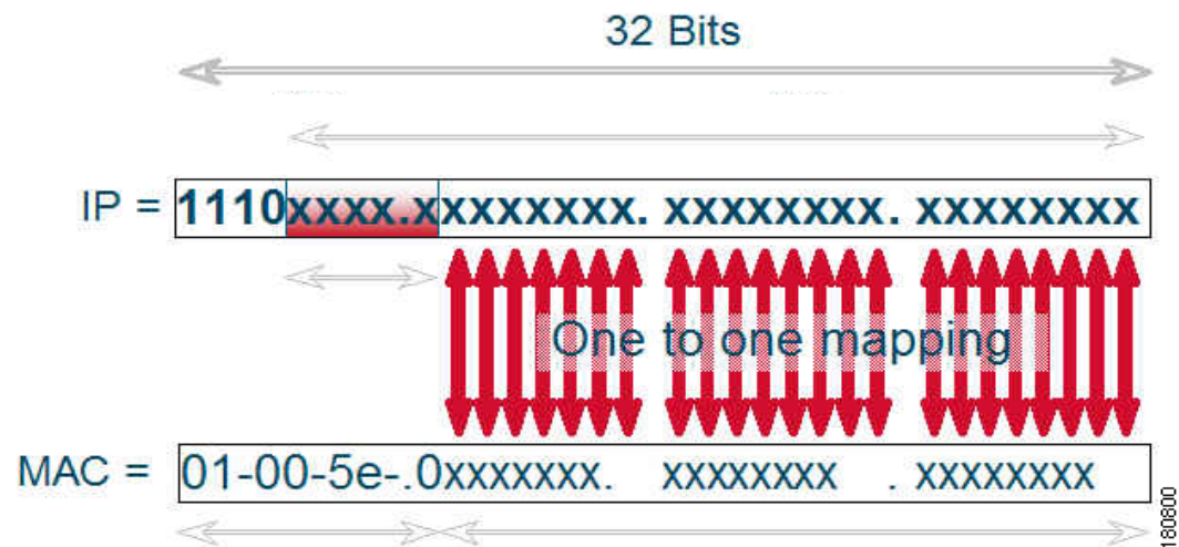
Figure 49-7 Multicast Addressing: Layer 3 to Layer 2 Mapping
