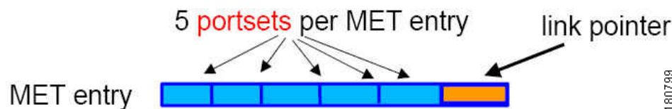
Figure 49-9 MET Entry Computations
