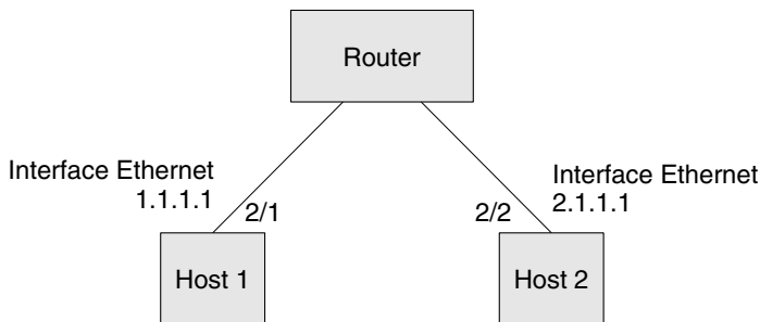
Figure 25-2 Physical Layer 3 Interfaces for the Catalyst 4500 Series Switch
