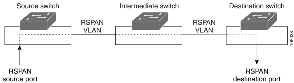
Figure 41-2 Example of RSPAN Configuration
