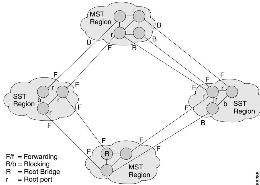
Figure 17-2 Network with Interconnected SST and MST Regions
