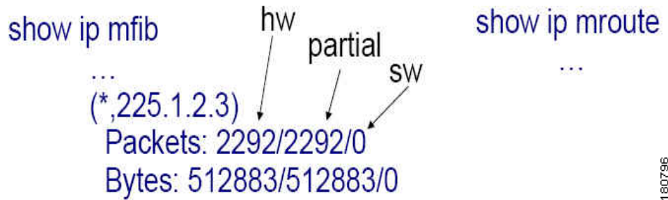
Figure 49-5 MFIB Entry: Counters
