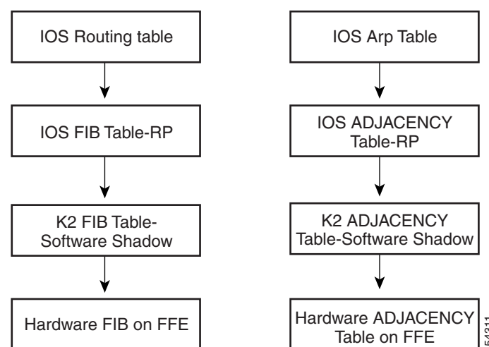
Figure 49-11 FIB Programming Flow
