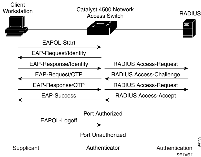
Figure 32-2 Message Exchange
