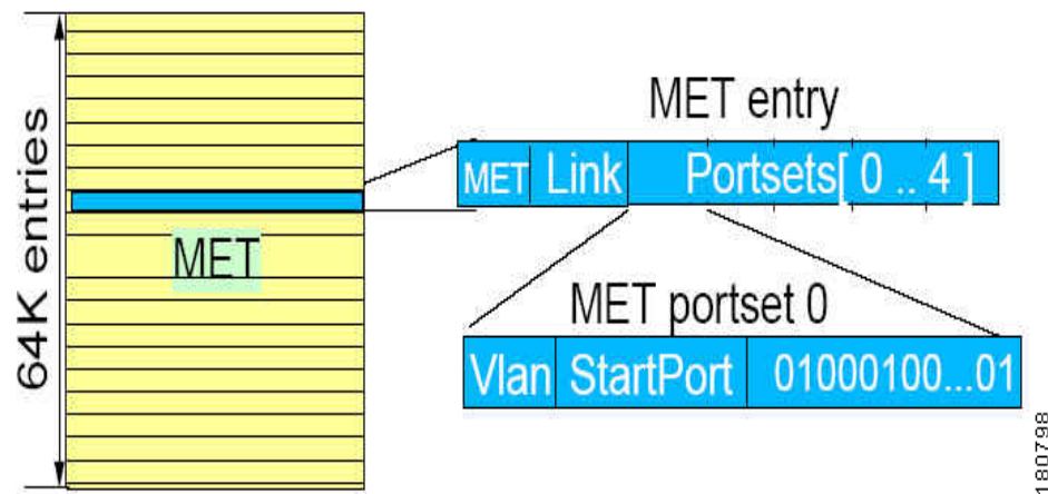
Figure 49-8 Multicast Expansion Table: Detail
