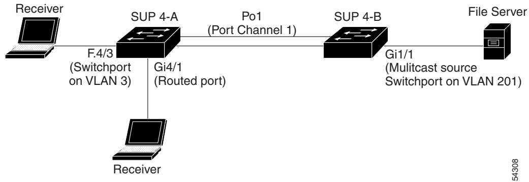
Figure 49-4 Topology - Multicast with Single Source and Multiple Receivers in Different VLANs
