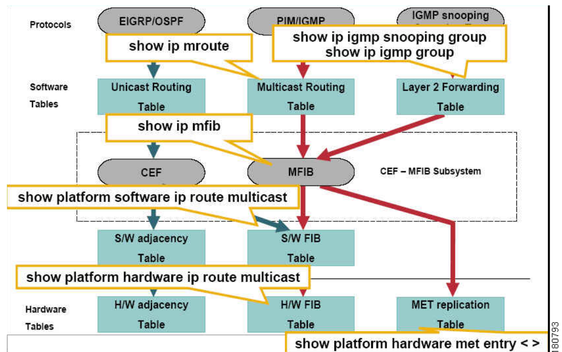
Figure 49-3 Multicast Programming Flow
