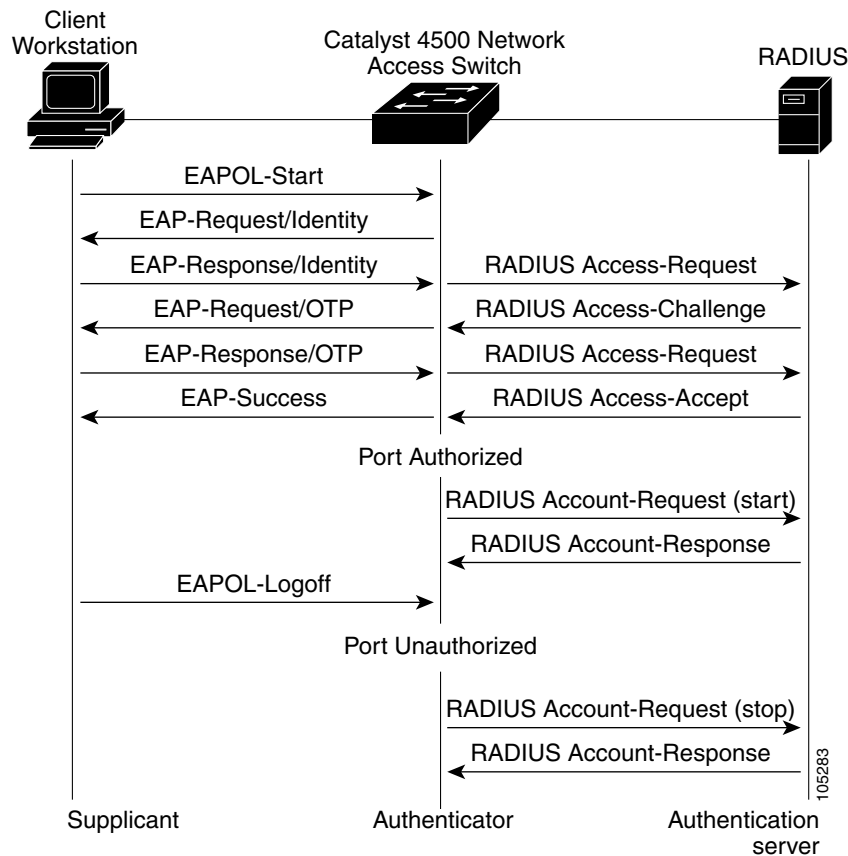
Figure 32-5 RADIUS Accounting
