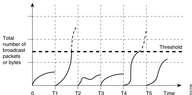
Figure 40-1 Storm Control Example - Hardware-based Implementation
