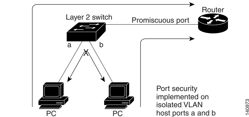
Figure 33-1 Port Security on Isolated Private VLAN Host Ports
