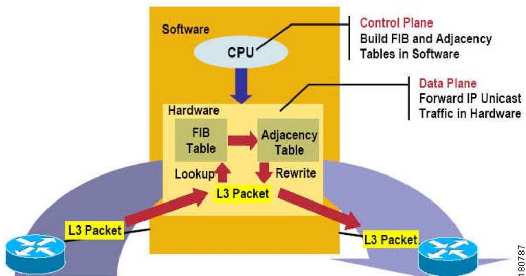
Figure 49-10 CEF-Based Unicast Forwarding
