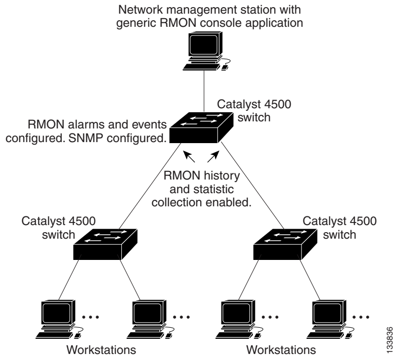
Figure 45-1 Remote Monitoring Example
