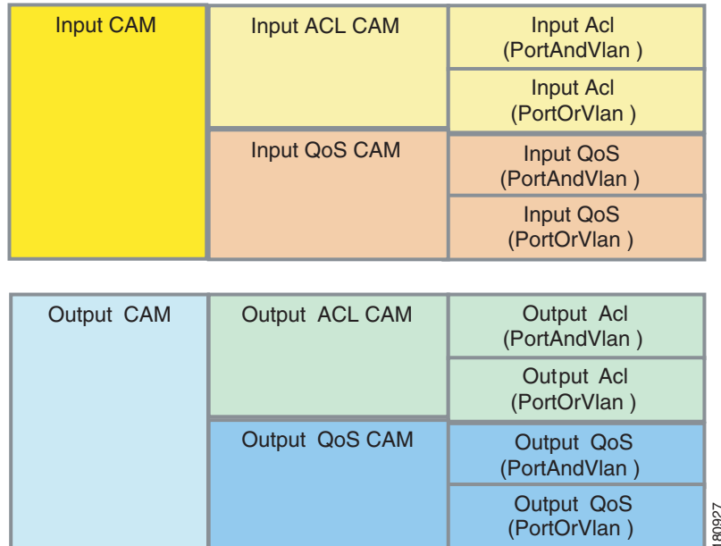
Figure 49-1 Structure of the Input and Output CAM
