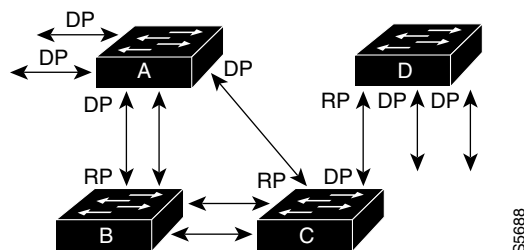
Figure 17-1 Spanning Tree Topology
