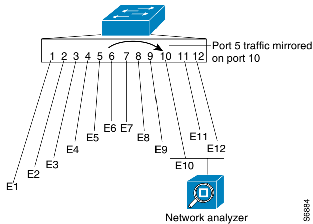
Figure 41-1 Example SPAN Configuration
