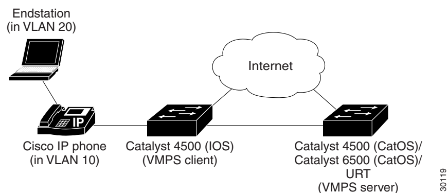
Figure 1-6 Dynamic Port VLAN Membership Configuration
