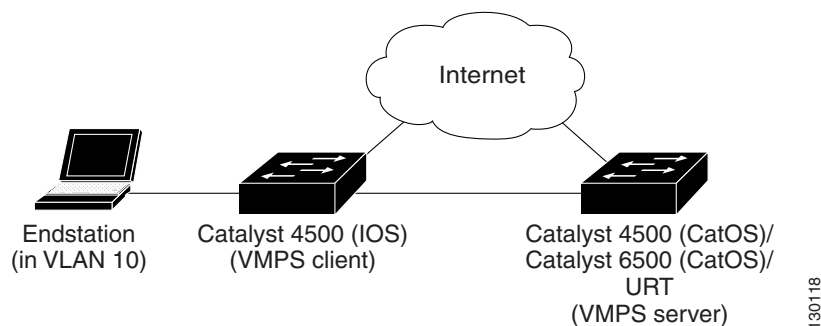
Figure 1-5 Dynamic Port VLAN Membership Configuration
