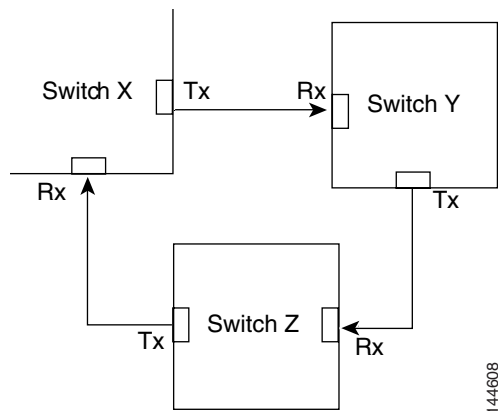
Figure 21-1 Unidirectional Link
