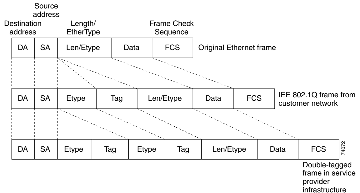
Figure 19-2 Original (Normal), 802.1Q, and Double-Tagged Ethernet Packet Formats
