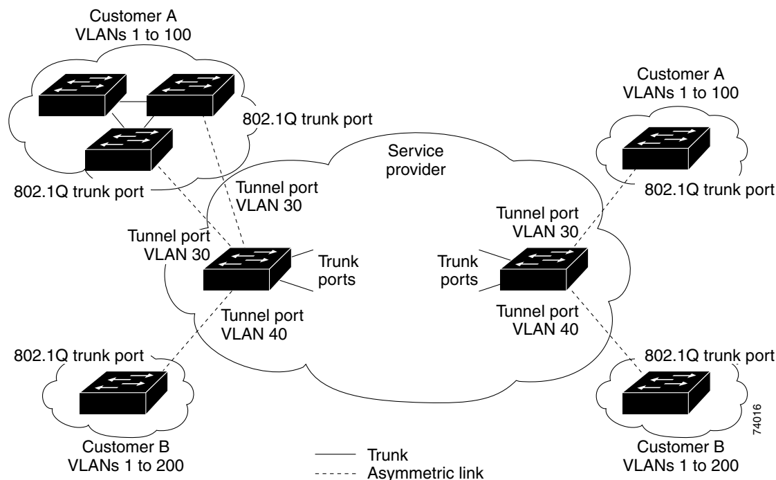
Figure 19-1 802.1Q Tunnel Ports in a Service Provider Network
