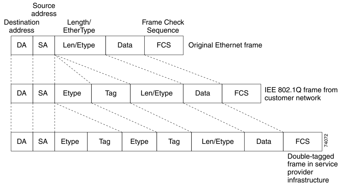
Figure 18-2 Original (Normal), 802.1Q, and Double-Tagged Ethernet Packet Formats
