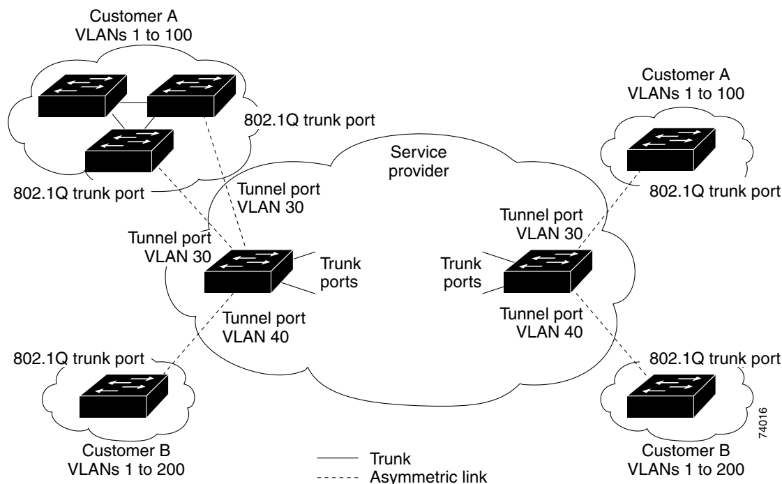
Figure 18-1 802.1Q Tunnel Ports in a Service Provider Network
