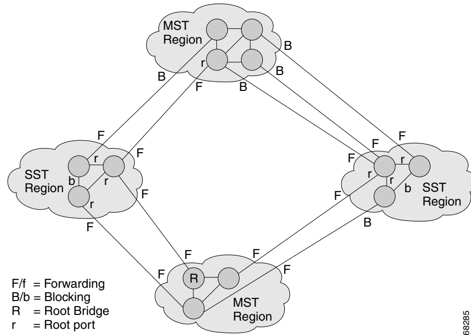
Figure 15-1 Network with Interconnected SST and MST Regions
