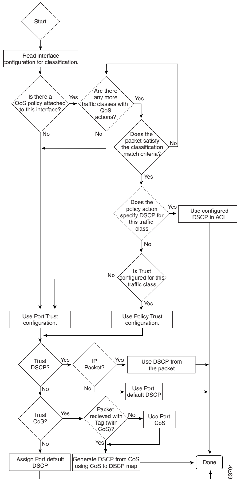
Figure 27-3 Classification Flowchart
