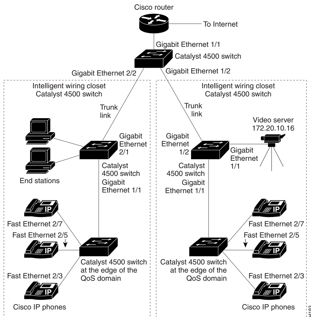
Figure 27-5 Auto-QoS Configuration Example Network
