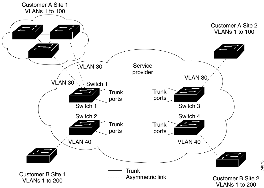
Figure 18-5 Layer 2 Network Topology without Proper Convergence
