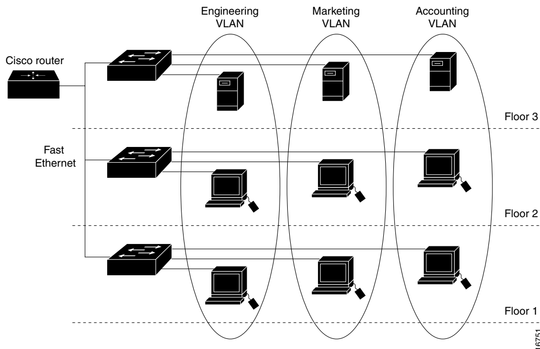
Figure 10-1 Sample VLANs
