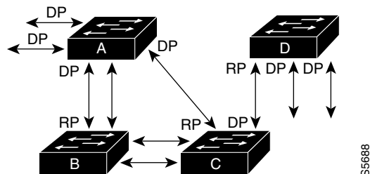
Figure 13-1 Spanning Tree Topology
