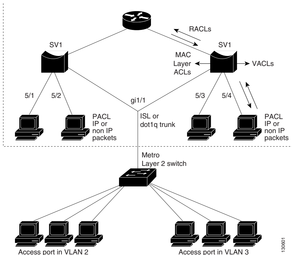
Figure 30-1 Trunk Port Security
