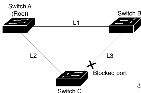
Figure 15-2 UplinkFast Before Direct Link Failure
