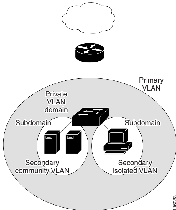
Figure 17-1 Private-VLAN Domain
