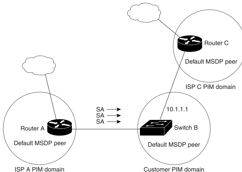
Figure 41-2 Default MSDP Peer Network
