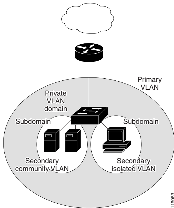
Figure 16-1 Private-VLAN Domain
