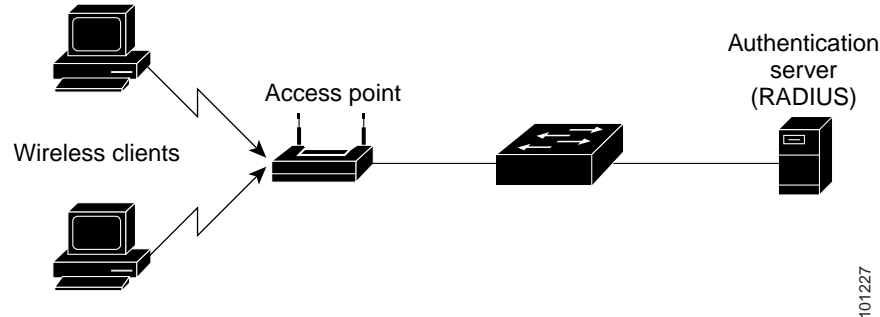
Figure 10-3 Multiple Host Mode Example
