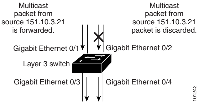
Figure 36-2 RPF Check
