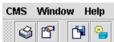
Figure 3-1 Menu Bar
