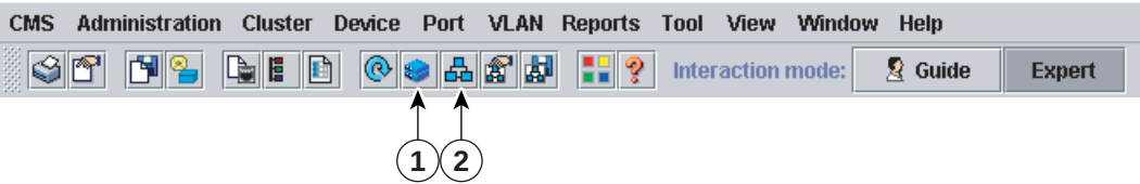
Figure 3-6 Toolbar
