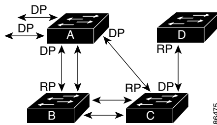
Figure 17-3 Spanning-Tree Topology
