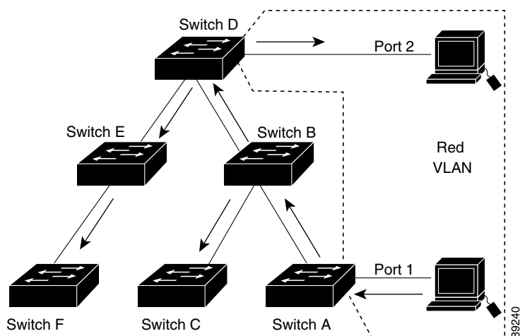
Figure 14-1 Flooding Traffic without VTP Pruning
