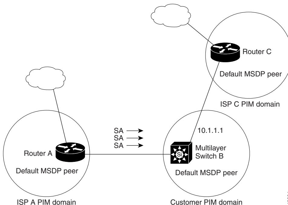
Figure 32-2 Default MSDP Peer Network
