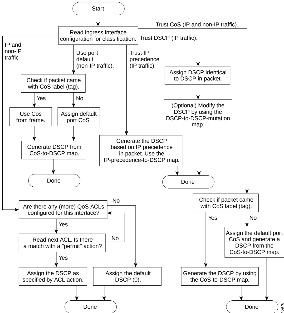
Figure 27-3 Classification Flowchart
