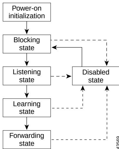
Figure 14-2 Spanning-Tree Interface States
