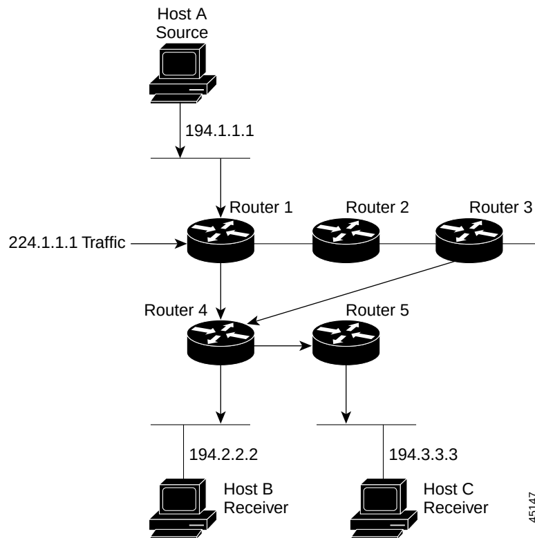
Figure 31-4 Host A Shortest-Path Tree
