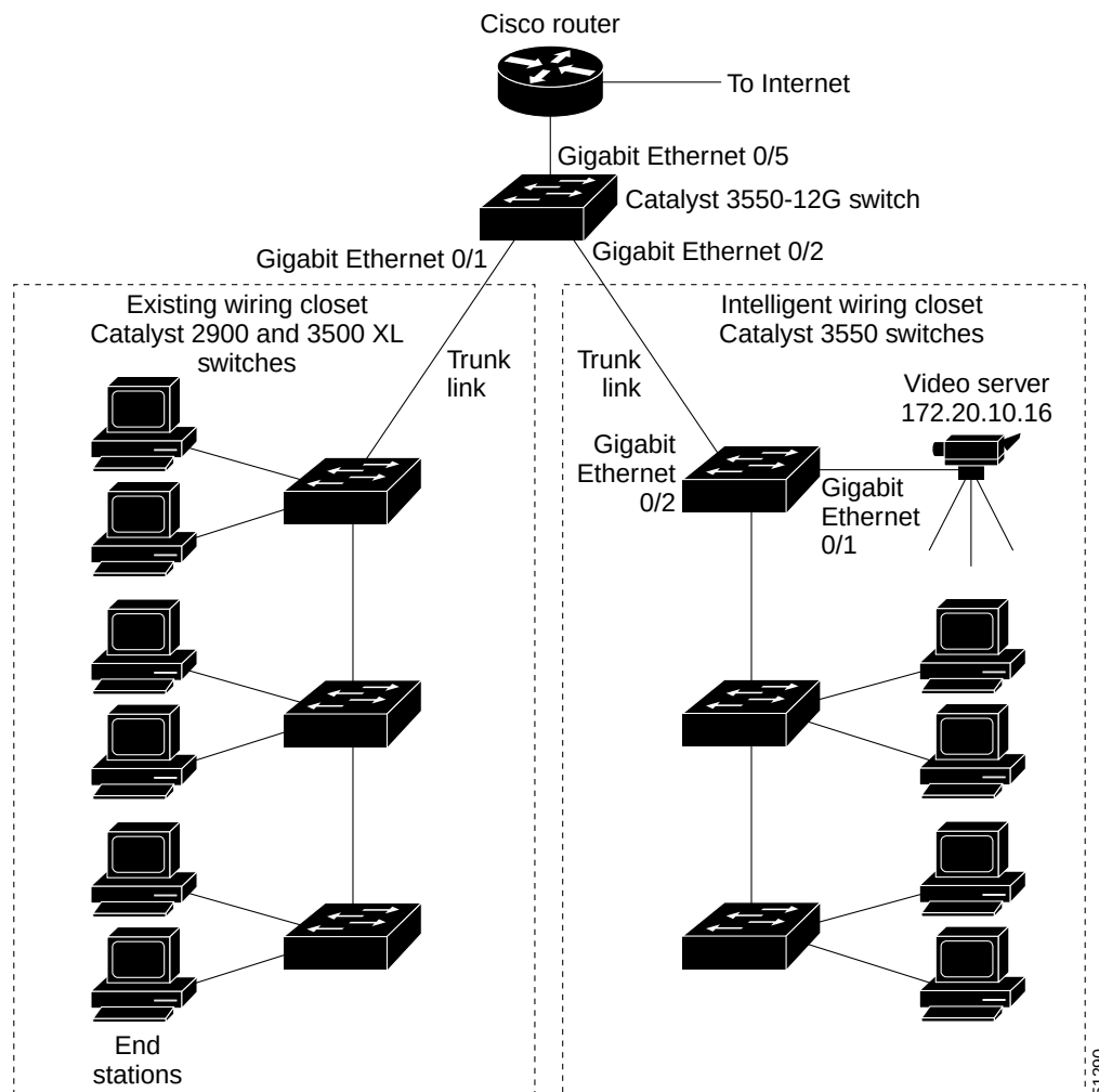
Figure 27-10 QoS Configuration Example Network
