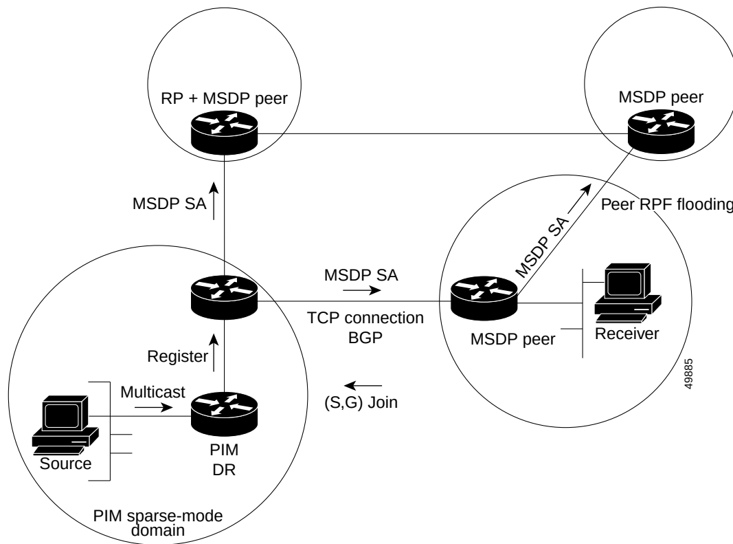
Figure 32-1 MSDP Running Between RP Peers
