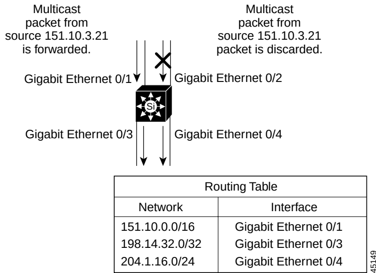
Figure 31-6 RPF Check
