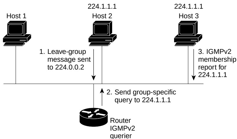
Figure 31-3 IGMPv2 Leave Process
