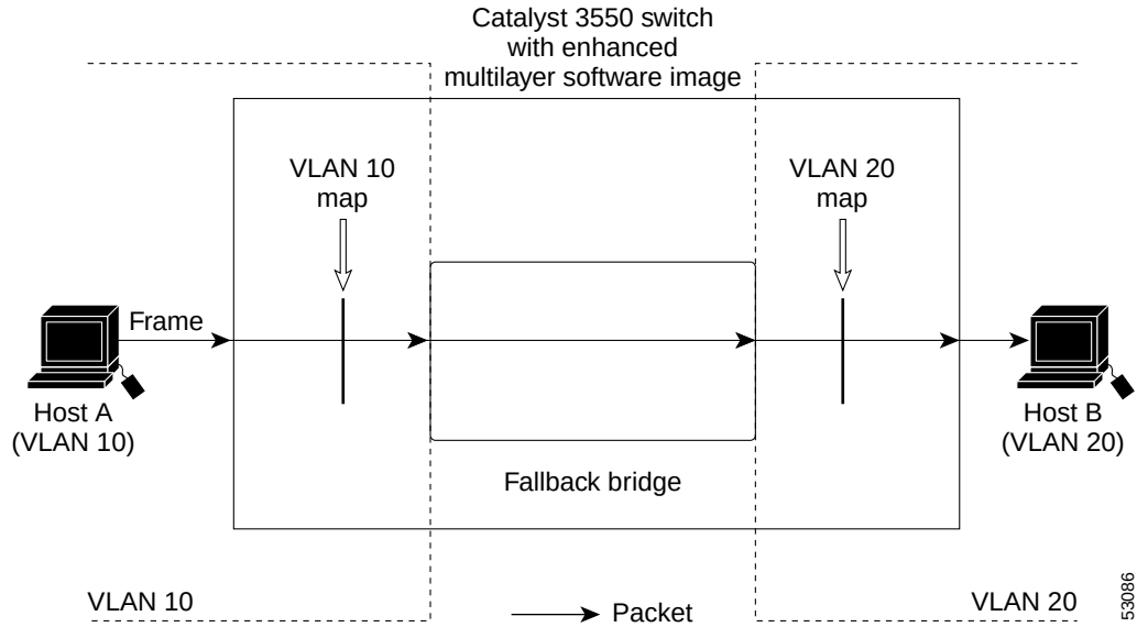
Figure 26-7 Applying ACLs on Bridged Packets
