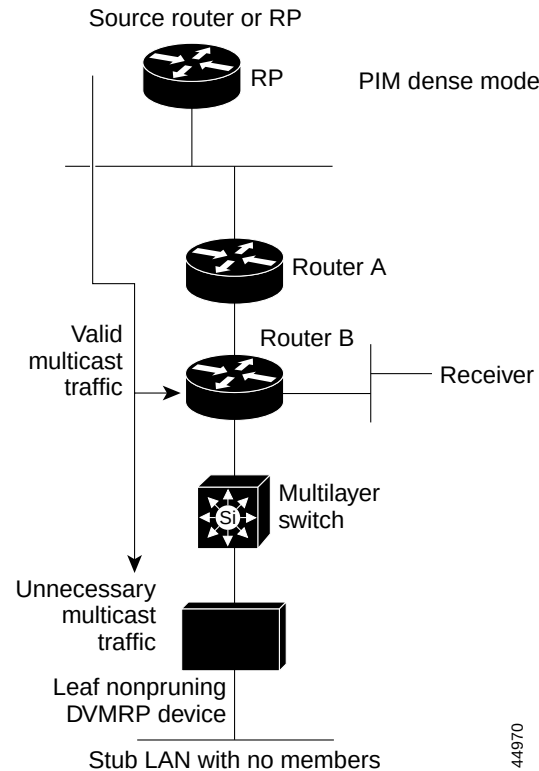
Figure 31-13 Leaf Nonpruning DVMRP Neighbor
