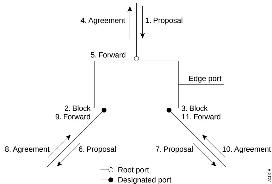
Figure 15-2 Sequence of Events During Rapid Convergence
