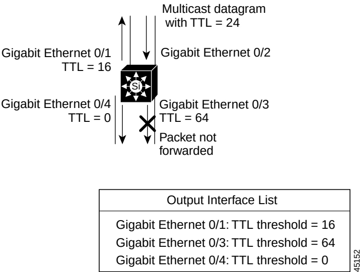
Figure 31-10 TTL Thresholds
