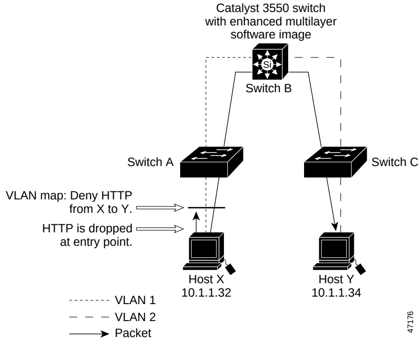
Figure 26-4 Wiring Closet Configuration
