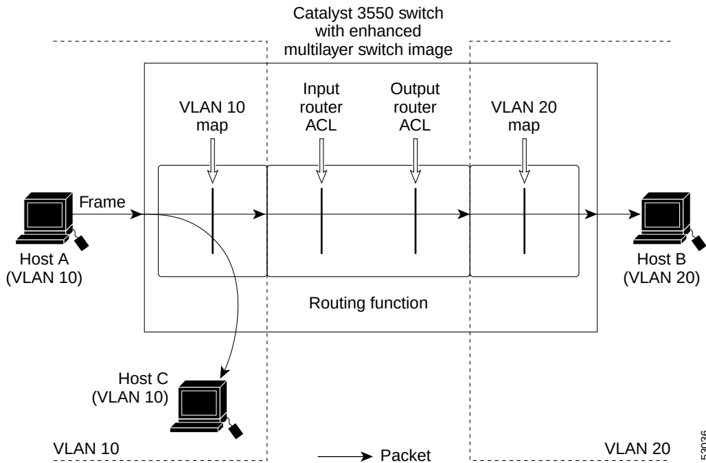
Figure 26-9 Applying ACLs on Multicast Packets
