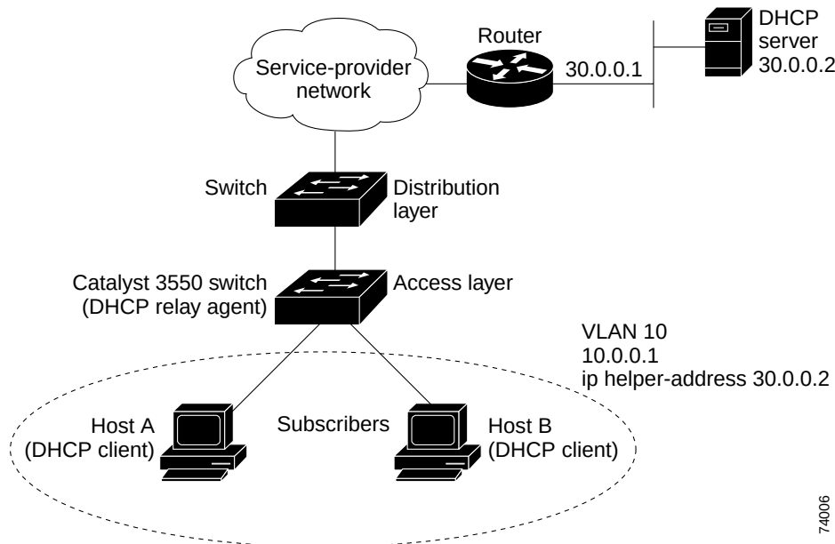
Figure 17-1 DHCP Relay Agent in a Metropolitan Ethernet Network
