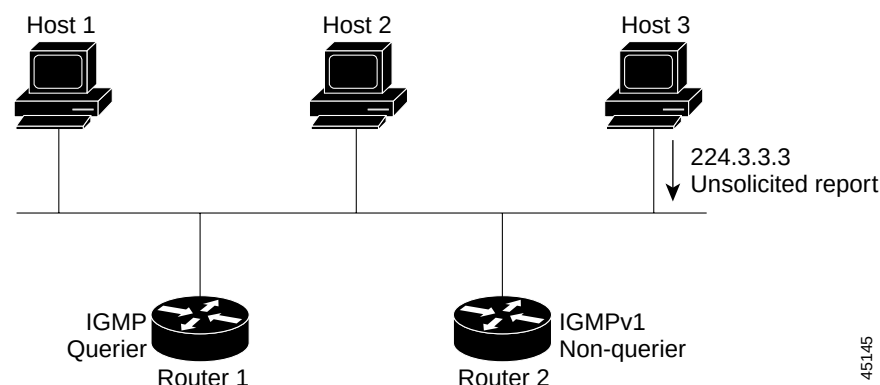
Figure 31-2 IGMPv1 Join Process
