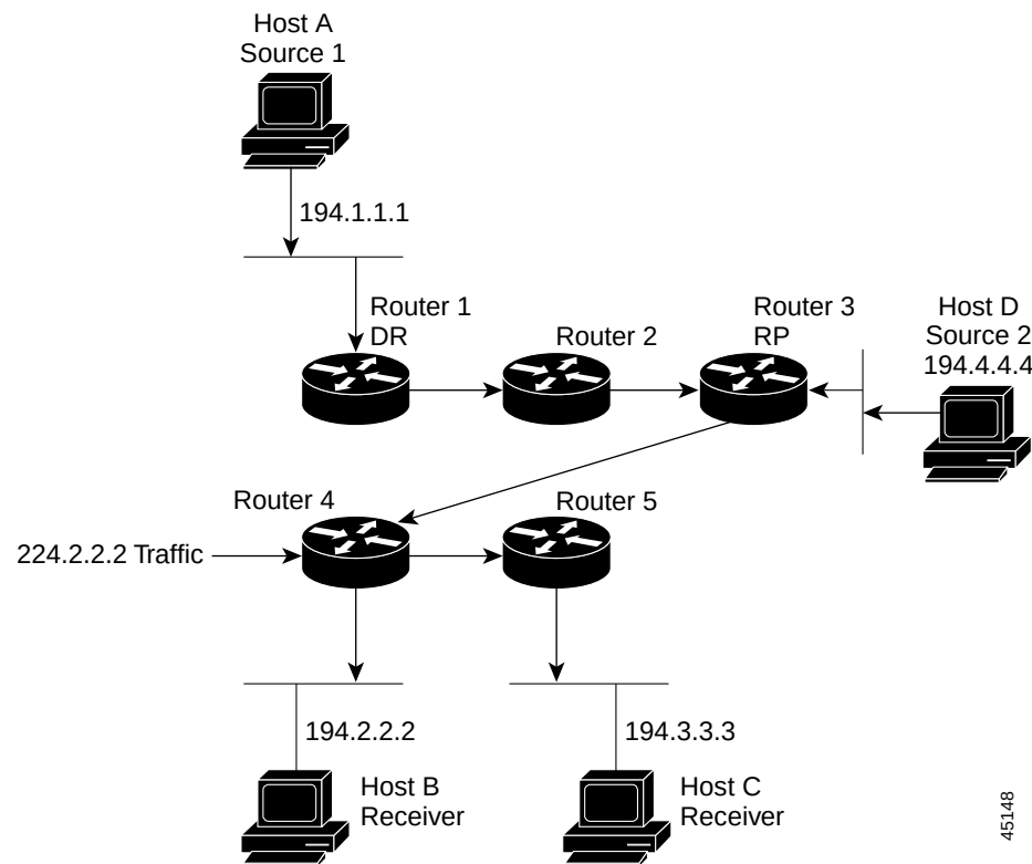
Figure 31-5 Shared Distribution Tree
