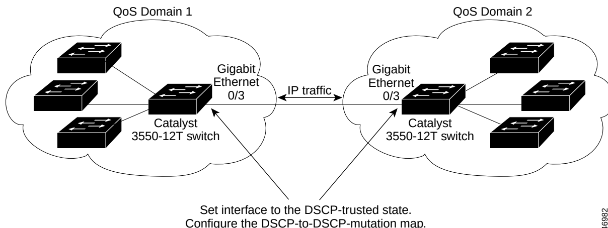
Figure 27-9 DSCP-Trusted State on a Port Bordering Another QoS Domain
