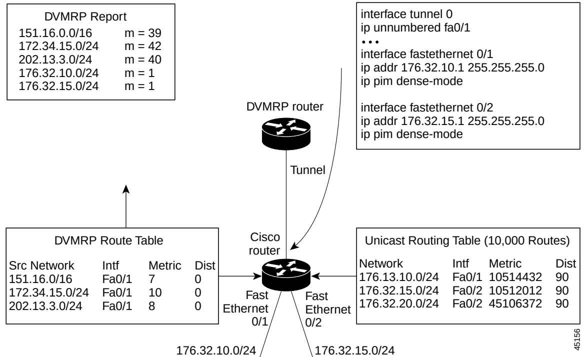
Figure 31-15 Only Connected Unicast Routes Are Advertised by Default
