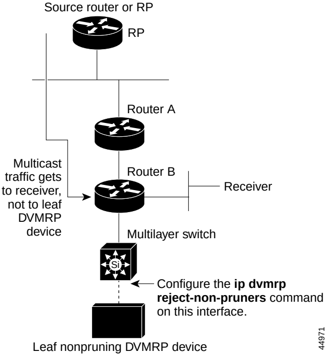
Figure 31-14 Router Rejects Nonpruning DVMRP Neighbor
