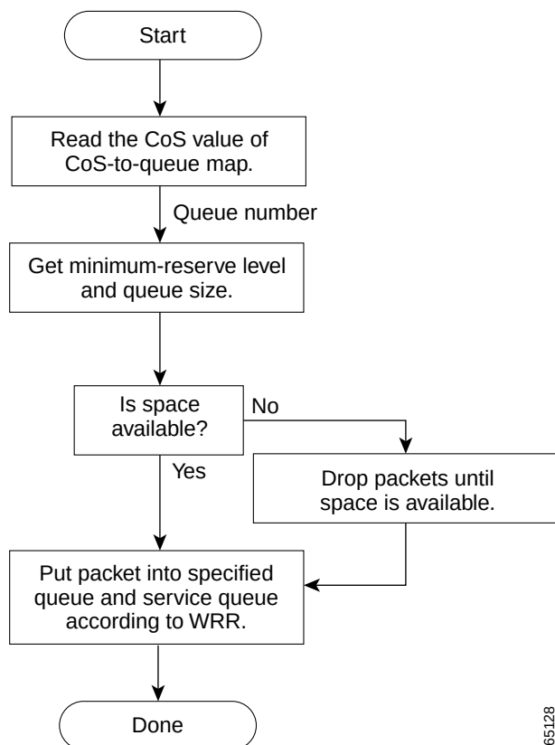
Figure 27-6 Queueing and Scheduling Flowchart for 10/100 Ethernet Ports
