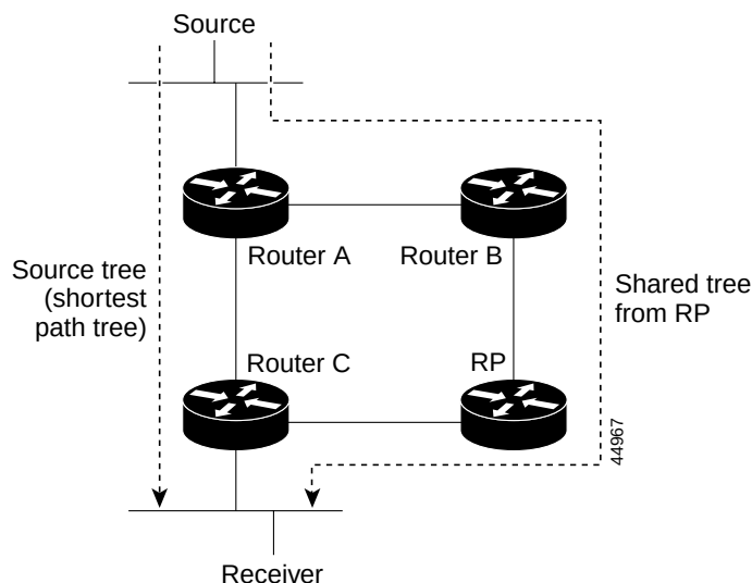
Figure 31-9 Shared Tree and Source Tree (Shortest-Path Tree)
