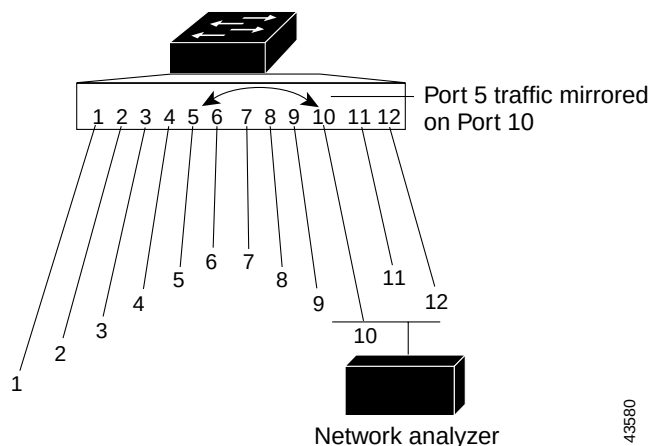
Figure 22-1 Example SPAN Configuration
