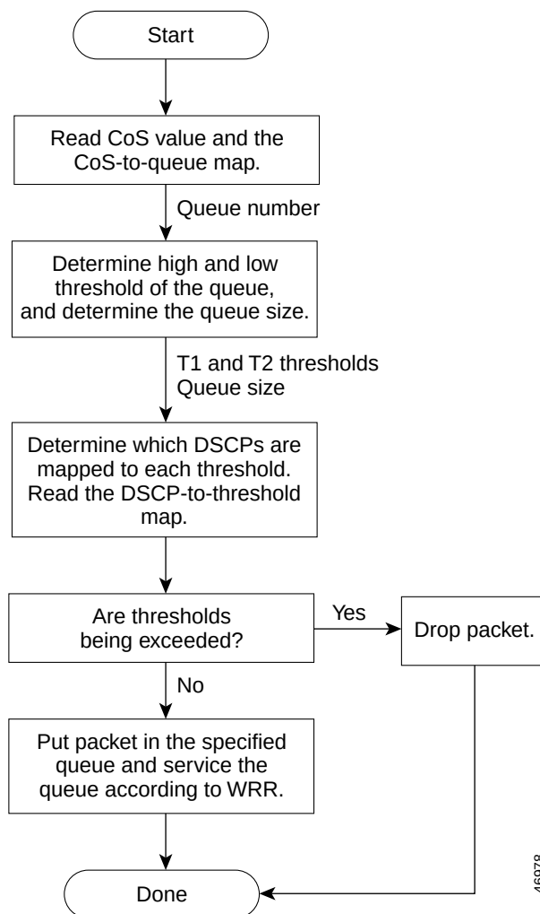
Figure 27-5 Queueing and Scheduling Flowchart for Gigabit-Capable Ethernet Ports
