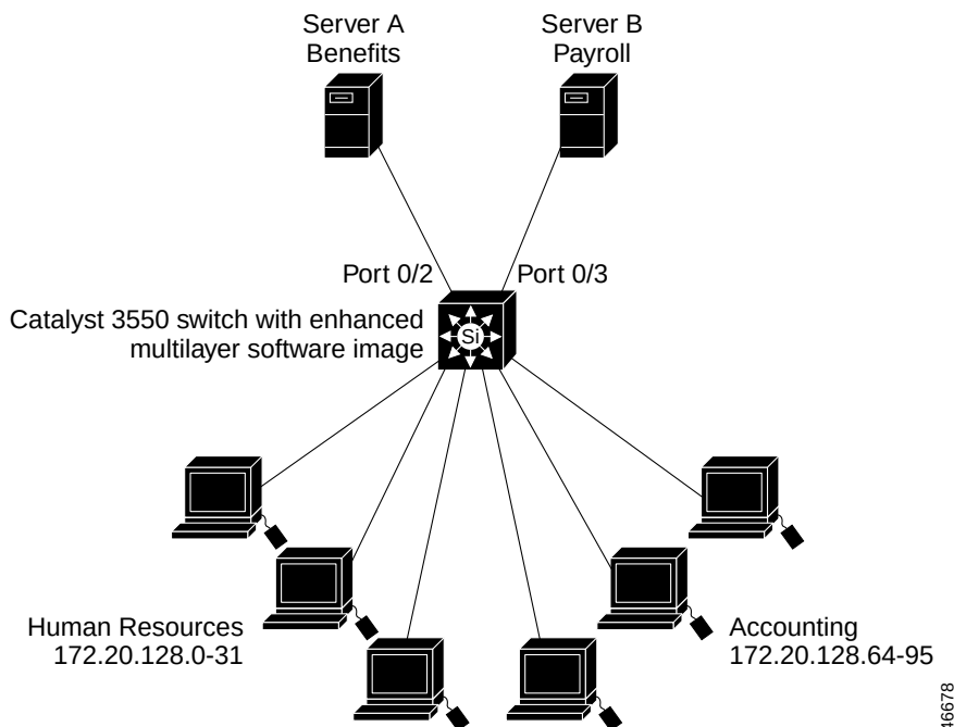
Figure 26-3 Using Router ACLs to Control Traffic
