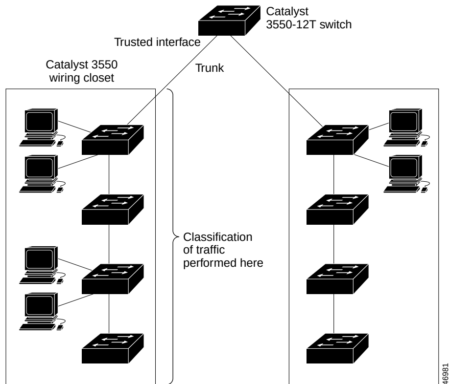
Figure 27-8 Port Trusted States within the QoS Domain
