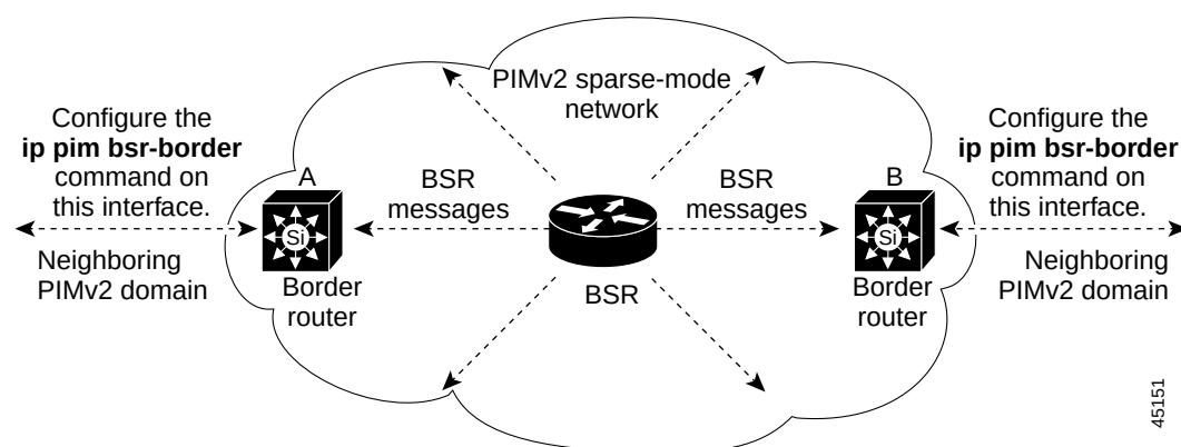
Figure 31-8 Constraining PIMv2 BSR Messages
