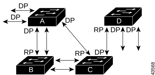
Figure 14-1 Spanning-Tree Topology
