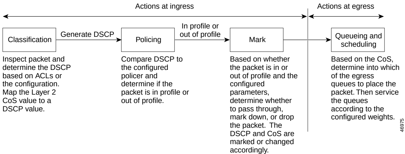
Figure 27-2 Basic QoS Model
