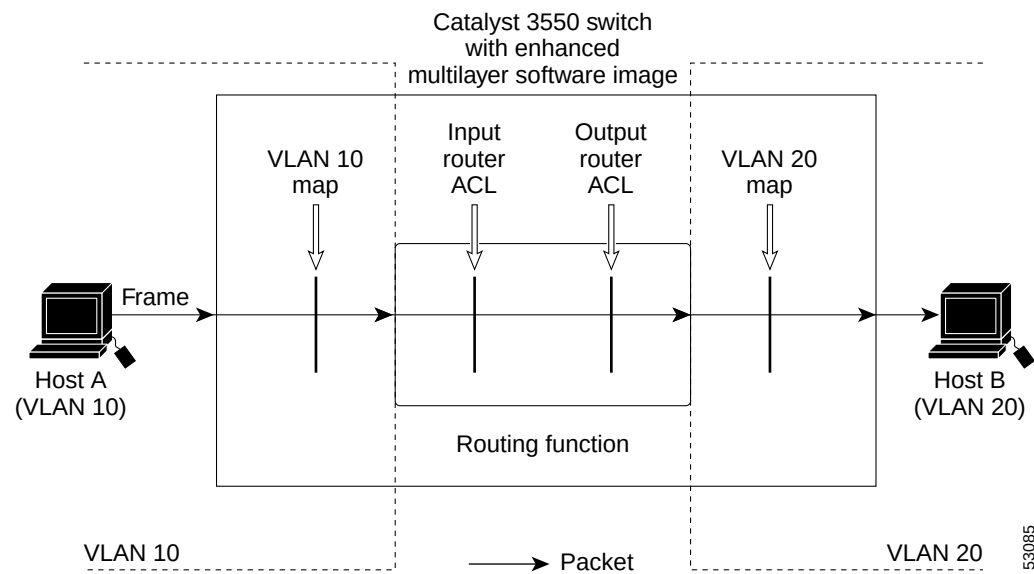
Figure 26-8 Applying ACLs on Routed Packets
