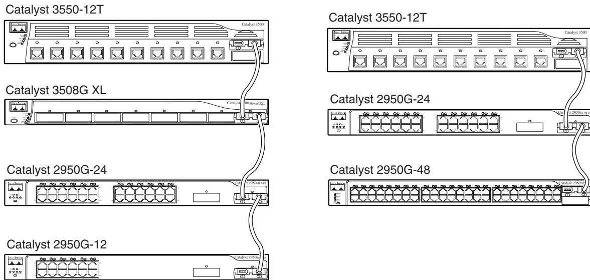
Figure 18-6 GigaStack GBIC Connections and Spanning-Tree Convergence
