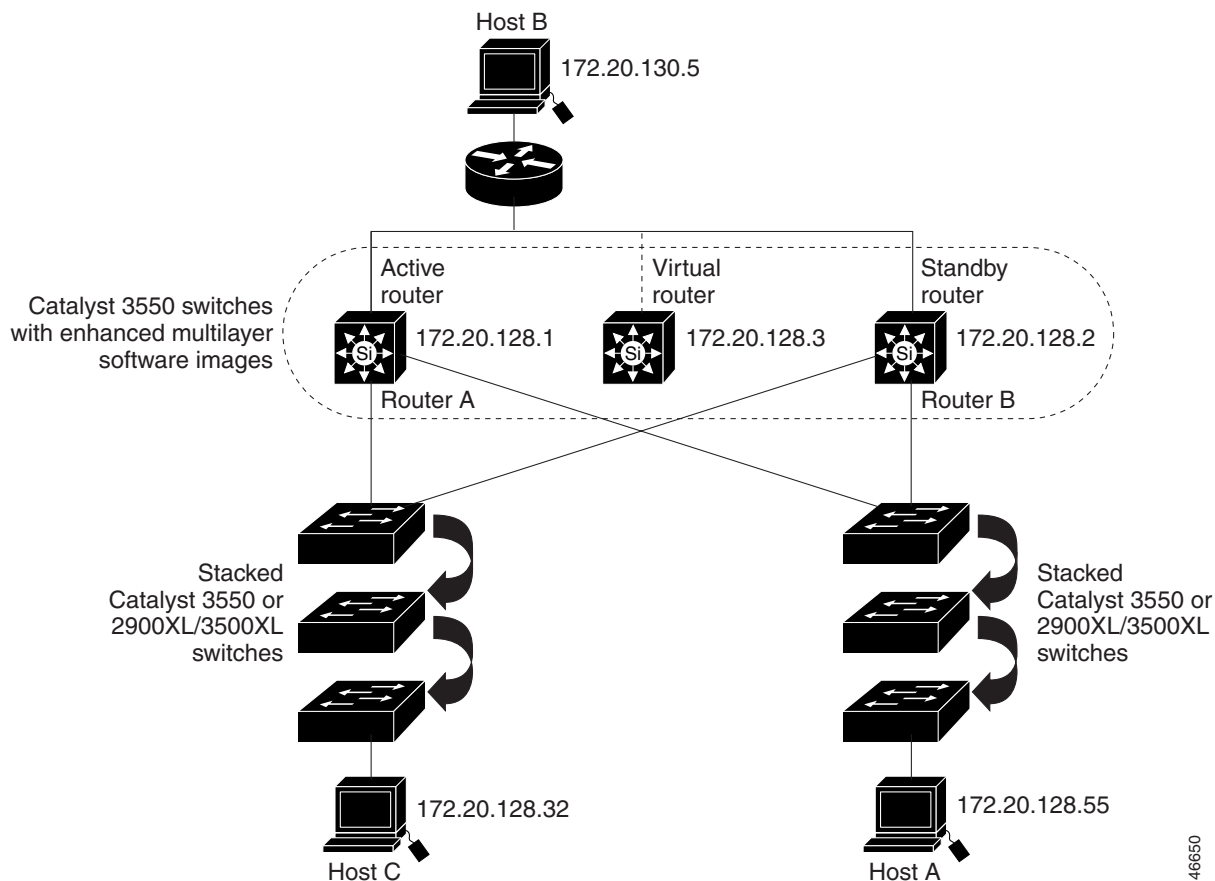
Figure 32-1 Typical HSRP Configuration
