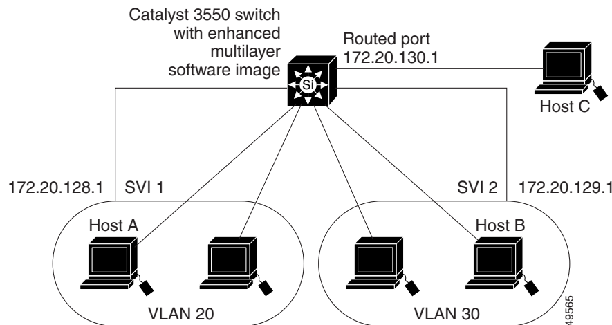
Figure 36-1 Fallback Bridging Network Example
