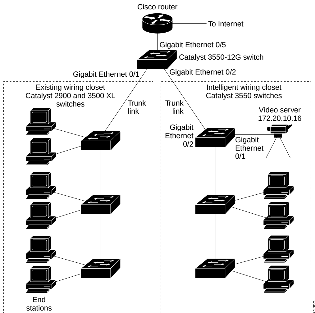
Figure 29-11 QoS Configuration Example Network
