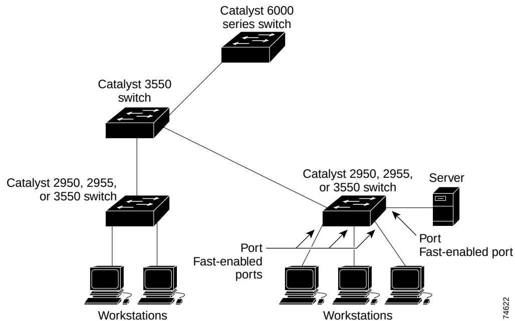
Figure 18-1 Port Fast-Enabled Ports
