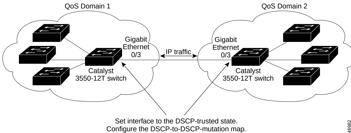
Figure 29-10 DSCP-Trusted State on a Port Bordering Another QoS Domain
