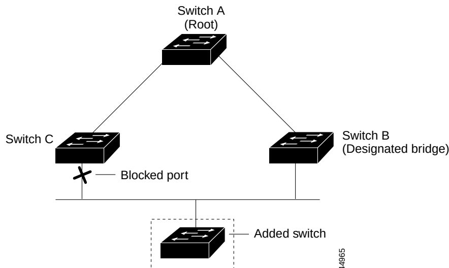
Figure 18-9 Adding a Switch in a Shared-Medium Topology
