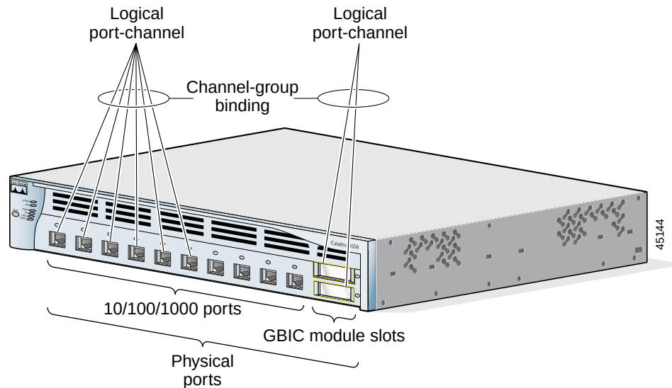
Figure 30-2 Relationship of Physical Ports, Logical Port Channels, and Channel Groups
