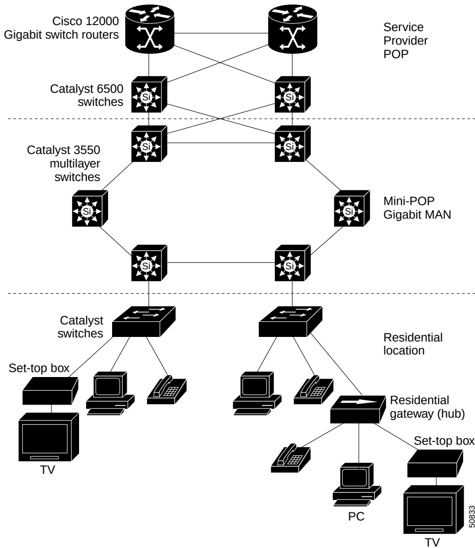
Figure 1-4 Catalyst 3550 Switches in a MAN Configuration
