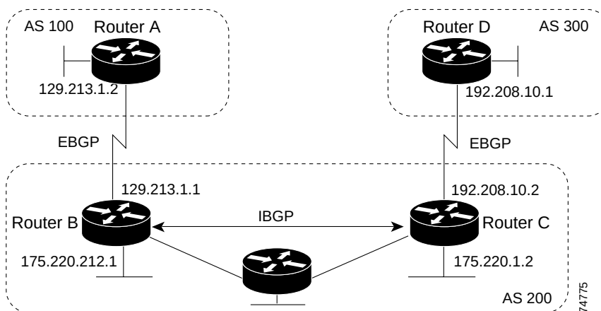
Figure 31-5 EBGP, IBGP, and Multiple Autonomous Systems
