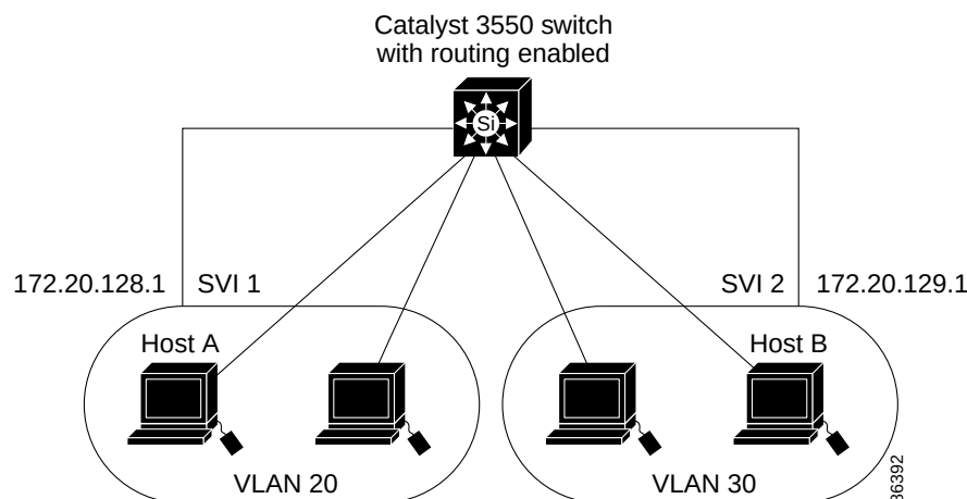
Figure 10-2 Connecting VLANs with the Catalyst 3550 Multilayer Switch
