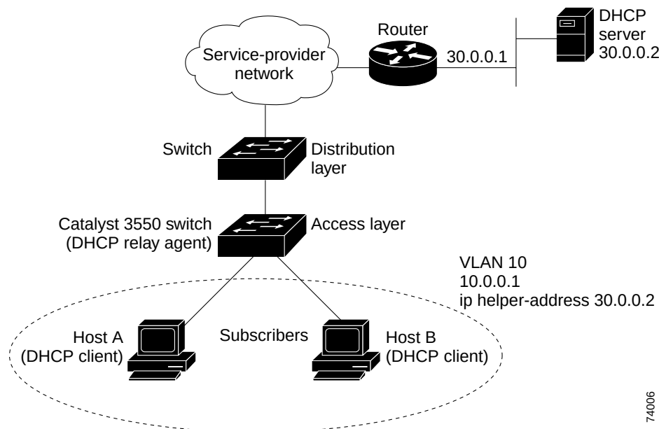
Figure 19-1 DHCP Relay Agent in a Metropolitan Ethernet Network
