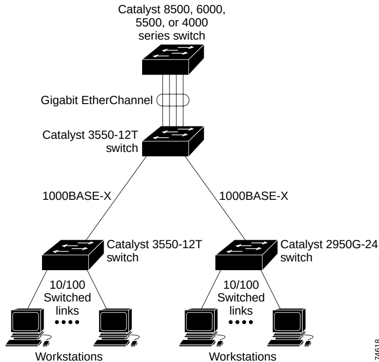
Figure 30-1 Typical EtherChannel Configuration
