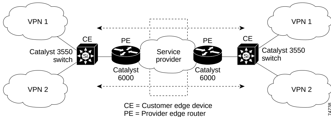
Figure 31-6 Catalyst 3550 Switches Acting as Multiple Virtual CEs
