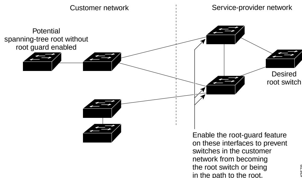
Figure 18-10 Root Guard in a Service-Provider Network
