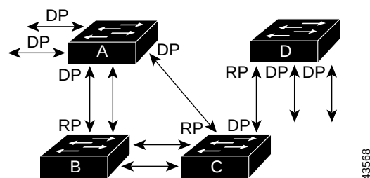
Figure 16-2 Spanning-Tree Topology
