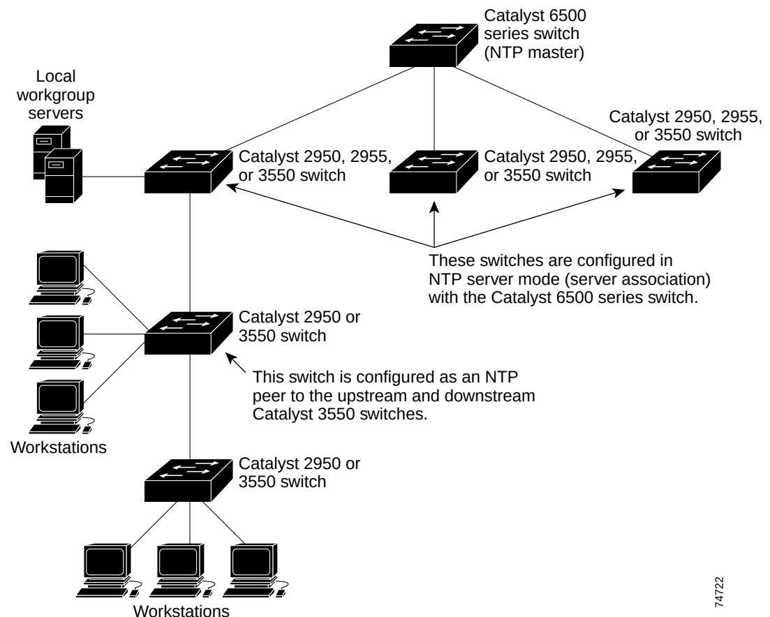
Figure 7-1 Typical NTP Network Configuration
