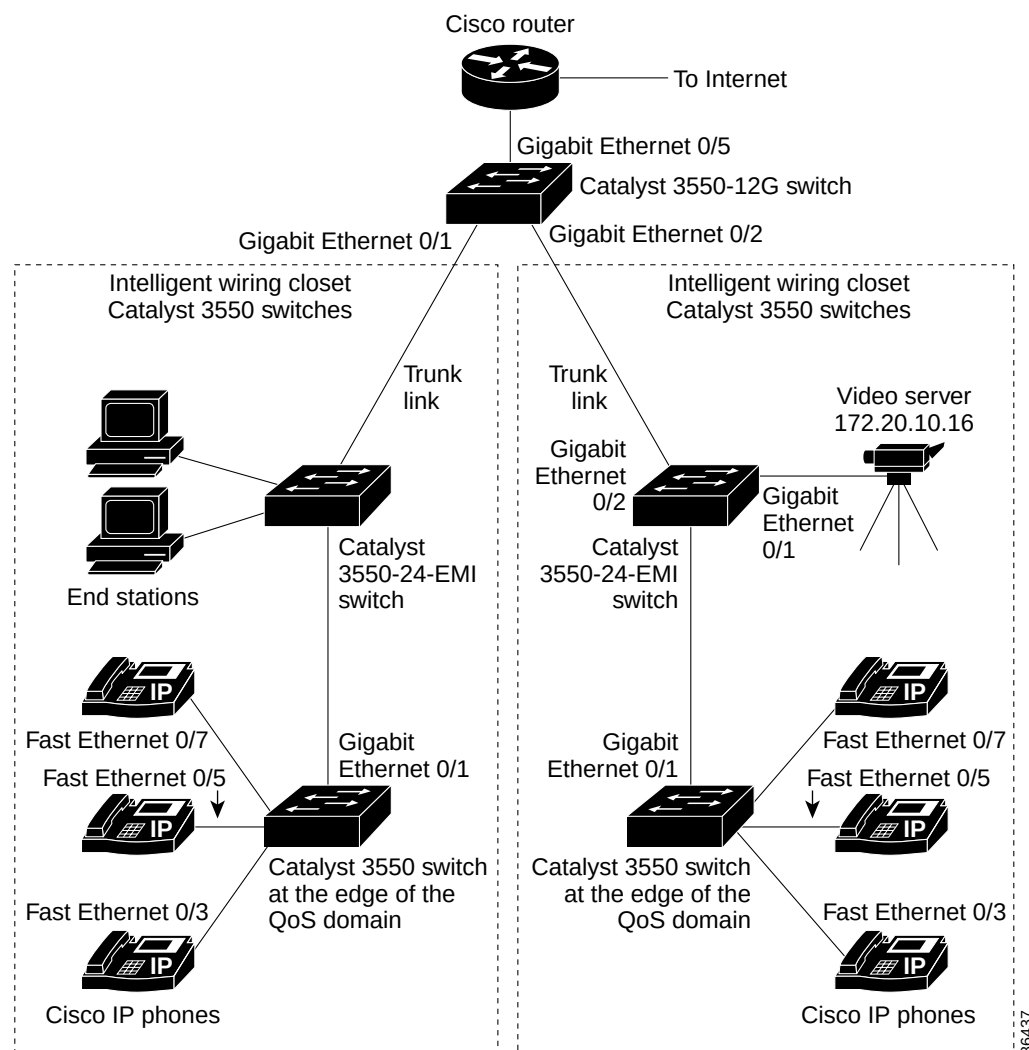
Figure 29-8 Auto-QoS Configuration Example Network
