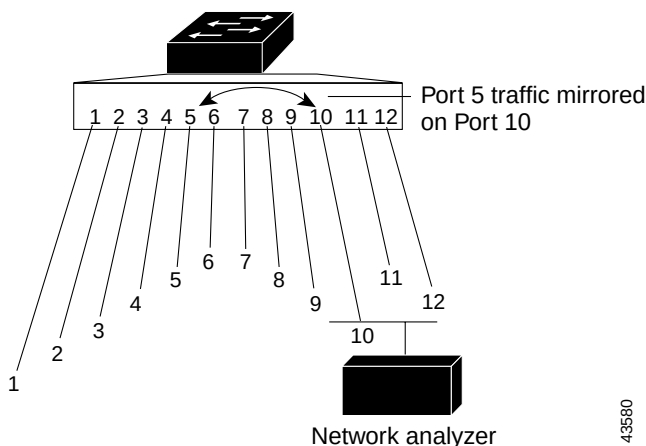
Figure 24-1 Example SPAN Configuration
