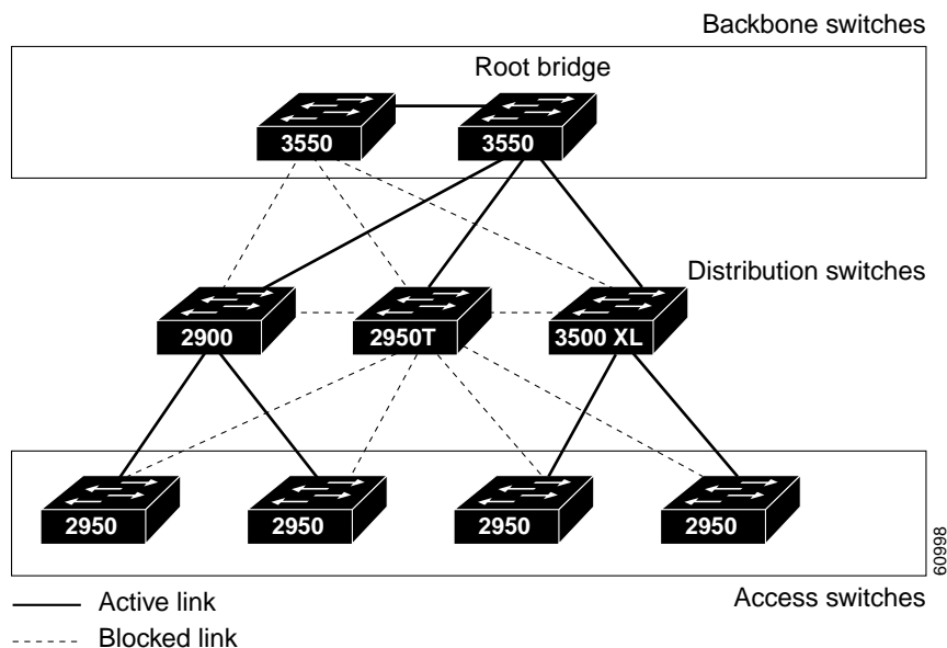
Figure 12-2 Switches in a Hierarchical Network
