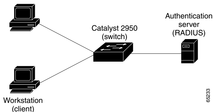
Figure 8-1 802.1X Device Roles
