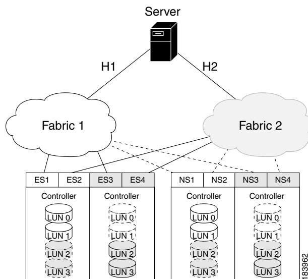
Figure 3-13 Example 1: Single LUN Set, Active-Passive Array
