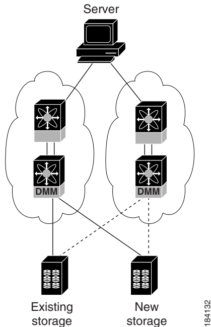
Figure 3-3 Homogeneous SAN Topolog
