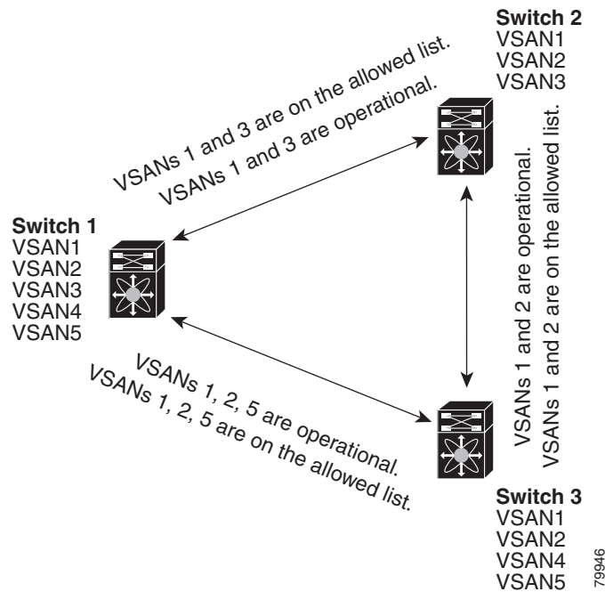
Figure 7-4 Operational and Allowed VSAN Configuration
