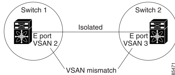
Figure 7-5 VSAN Mismatch
