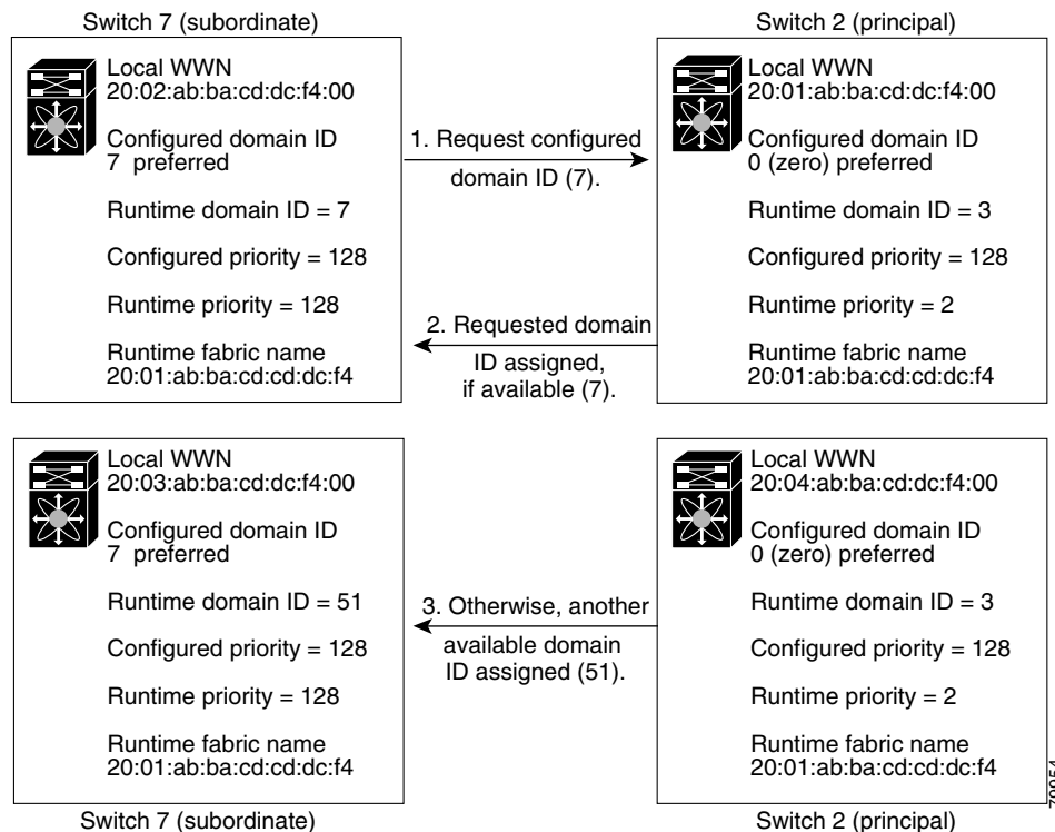
Figure 10-11 Configuration Process Using the preferred Option
