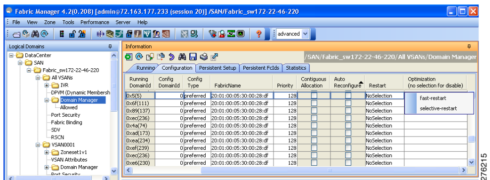
Figure 10-3 Configuring Domains
