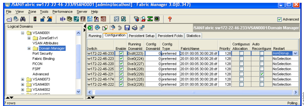
Figure 10-9 Configuring Domains
