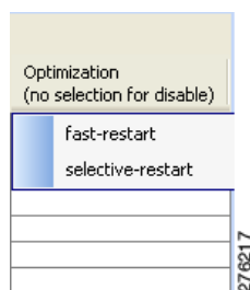
Figure 10-5 Optimization Field
