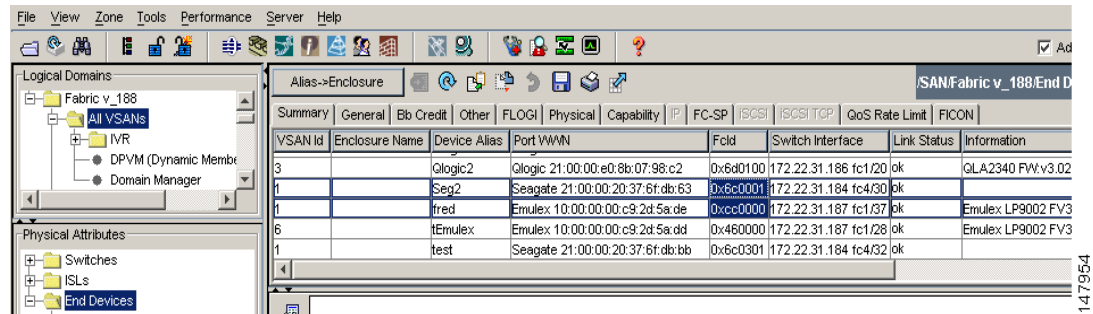
Figure 10-15 FLOGI Database Information in Fabric Manager
