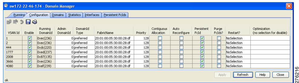
Figure 10-4 Configuring Domains
