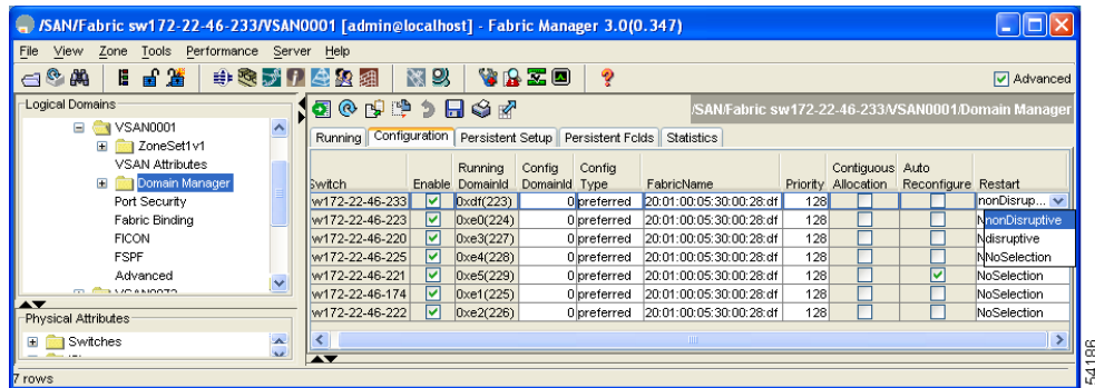
Figure 10-7 Configuring Domains
