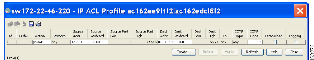
Figure 5-4 IP ACL Profile Dialog Box
