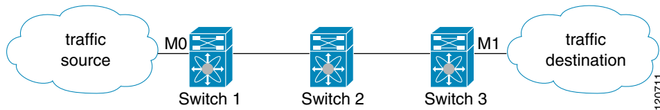
Figure 5-6 Denying Traffic on the Inbound Interface
