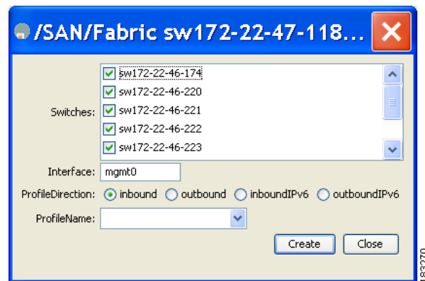
Figure 5-7 Create Interfaces Dialog Box
