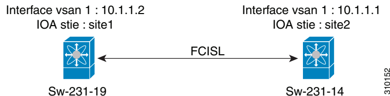
Figure 2-1 Configuration Example
