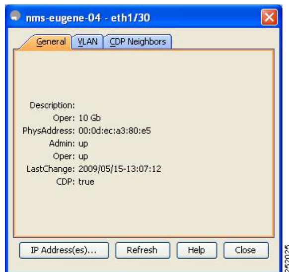
Figure 3-2 Ethernet Interfaces Dialog Box
