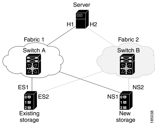
Figure 7-1 Example Topology
