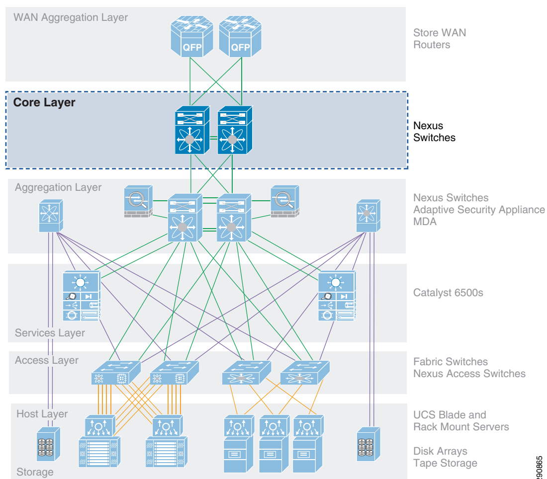
Figure 3-7 Core Layer
