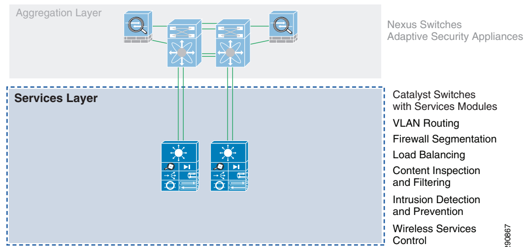
Figure 3-10 Services Layer
