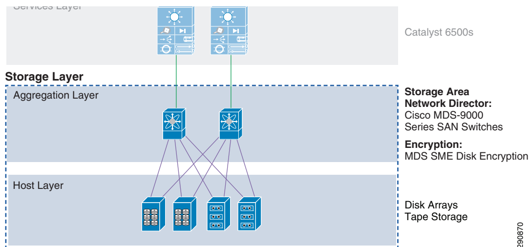
Figure 3-13 Storage Layer
