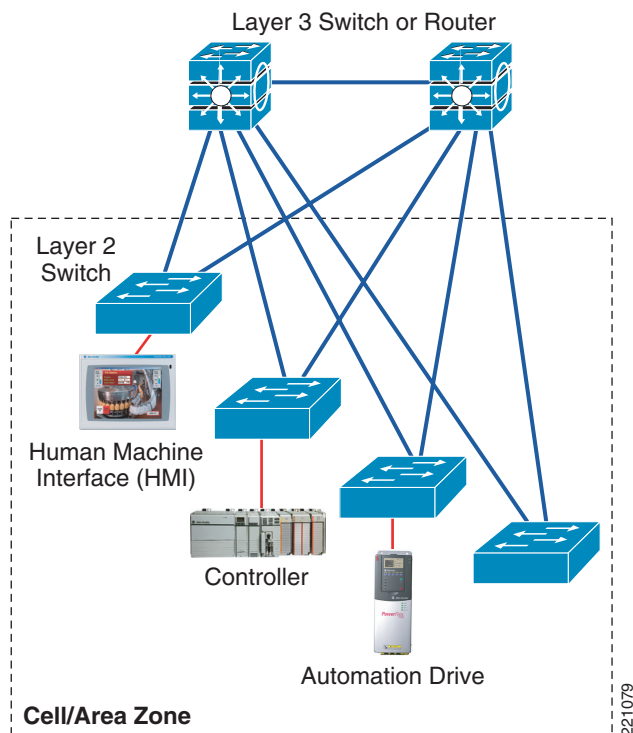
Figure 1-3 Star Topology
