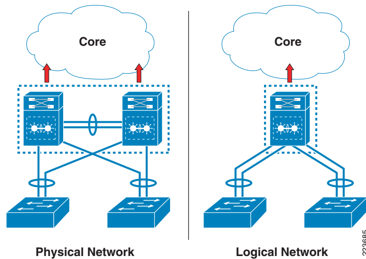
Figure 4 Cisco's Virtual Switching Systems
