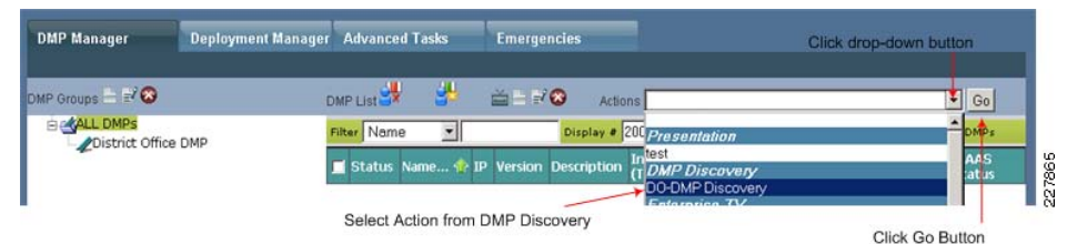
Figure 13 Triggering DMP Discovery Manually
