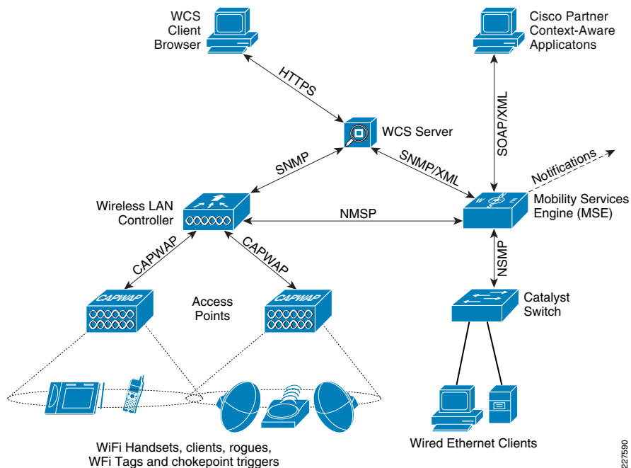
Figure 3 Protocol Interaction Between Context-Aware Components
