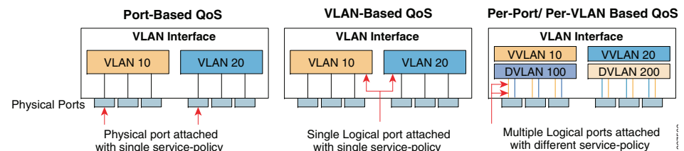
Figure 7 Depicts All Three QoS Implementation Method
