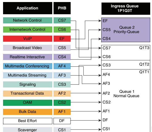
Figure 8 Ingress Queueing
