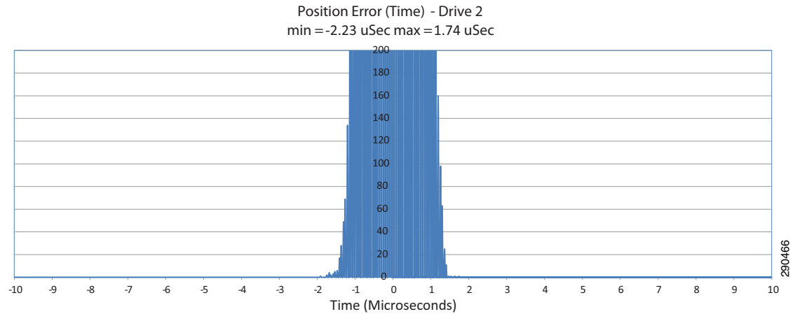
Figure 8-56 Star Architecture Offset to Master Test 2.1—Test @ Nominal Ixia Traffic Load
