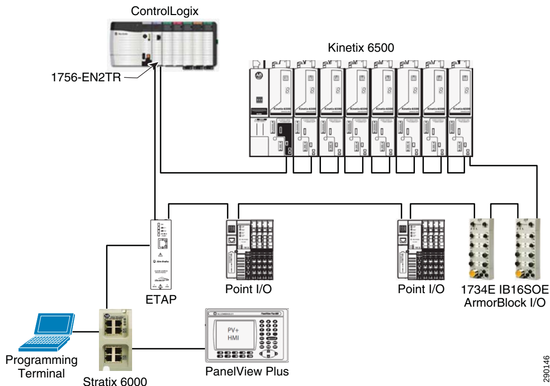
Figure 8-18 DLR Ring Reference Architecture
