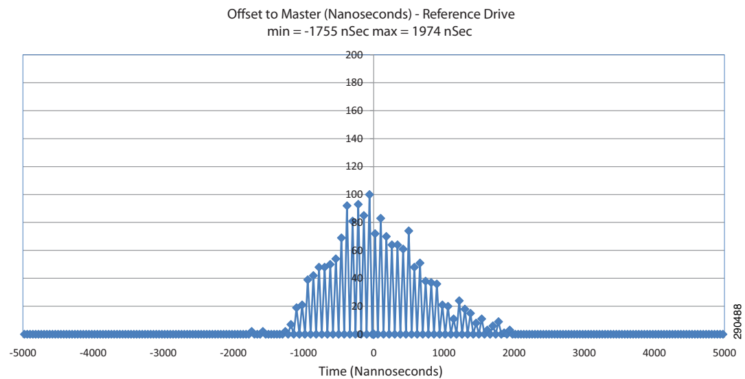
Figure 8-78 DLR Architecture Phase Error Test 0.3—Test @ 20% IX.IA Traffic Load
