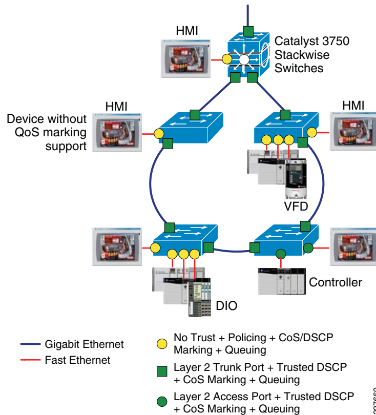
Figure 3-28 QoS Trust/No-Trust in Cell/Area Zone
