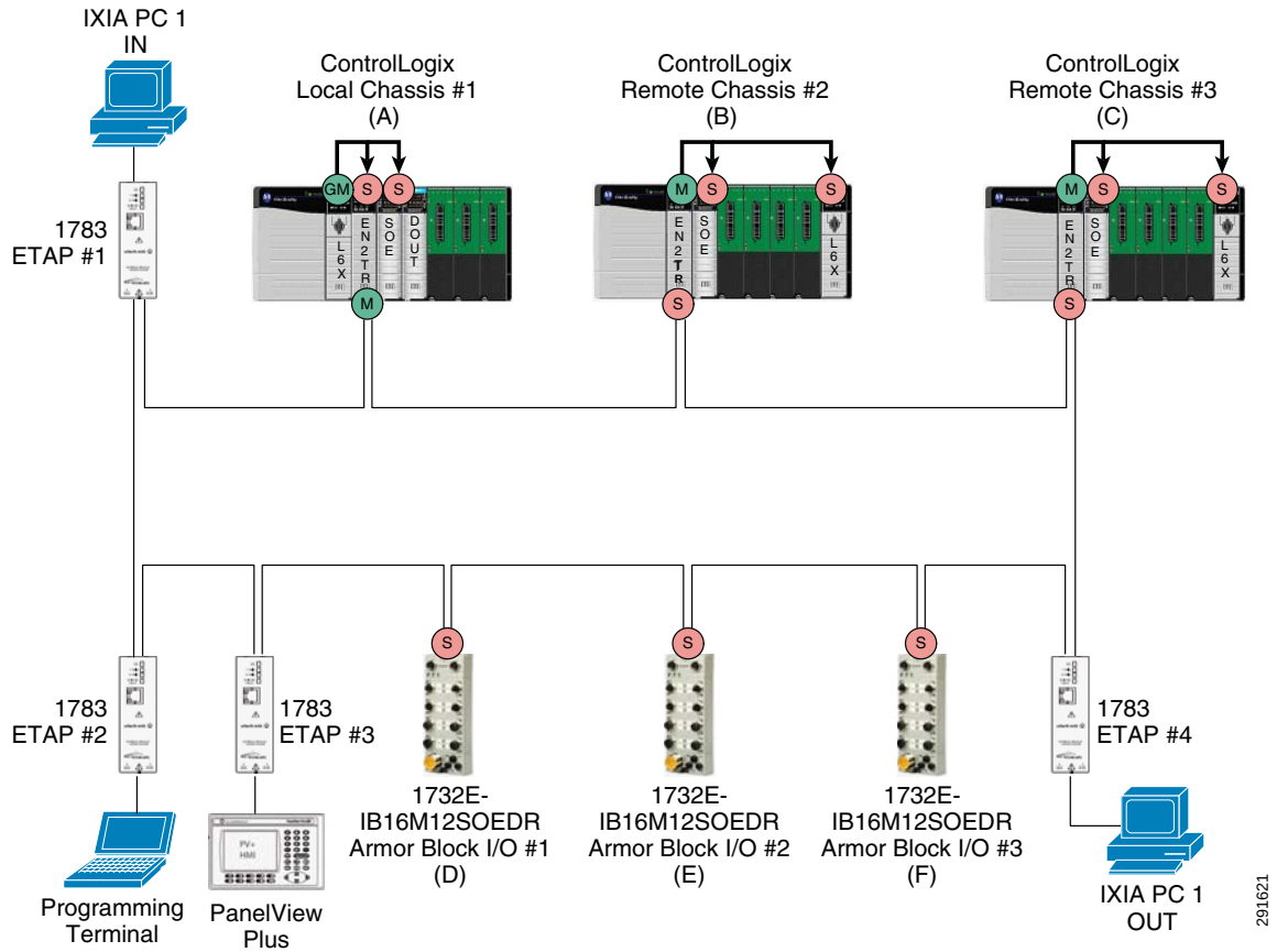
Figure 9-38 Ring Topology Using Embedded Dual-Port Ethernet Switch Devices with Transparent Clock
