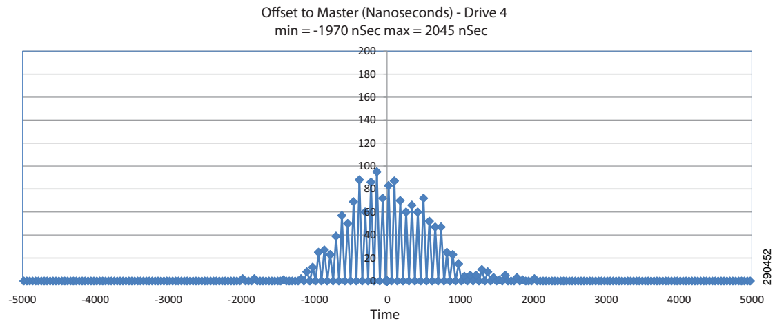
Figure 8-41 Linear Architecture Offset to Master Test 1.2—Test @ 10% Ixia Traffic Load
