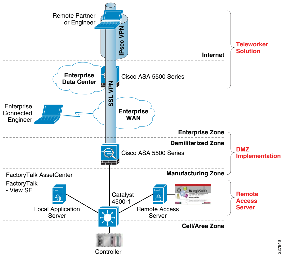
Figure 6-3 Simplified Remote Access
