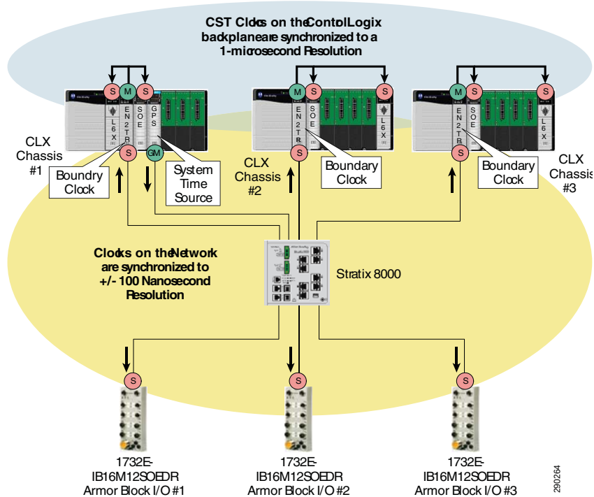
Figure 9-8 SOE Control System with a 1756HP-Time (GPS) Module Used as the Real-Time Source and the Grandmaster of the Ethernet Network
