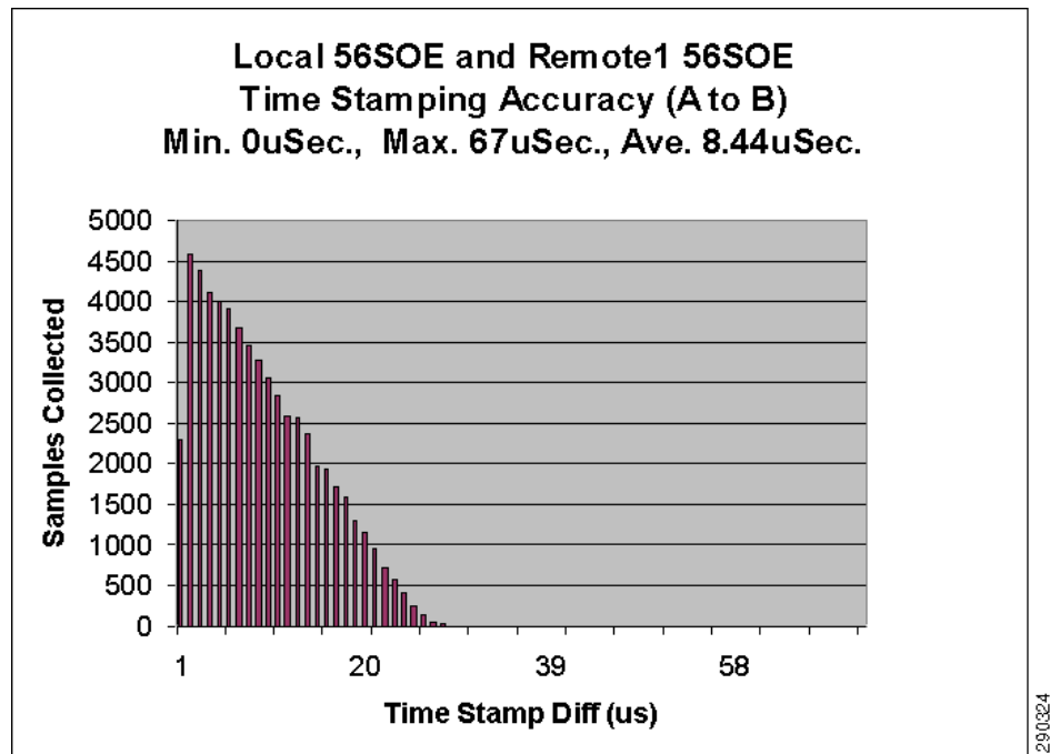
Figure 9-43 Multiple Star Topology—SOE Timestamp Test 3 Results Using 1756-EN2T Modules with Boundary Clock and Stratix 8000 Switch with Transparent Clock (A to B)
