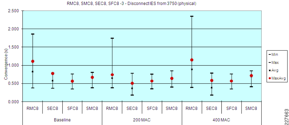
Figure 3-20 Network Convergence Test Results—Copper Uplink Topologies
