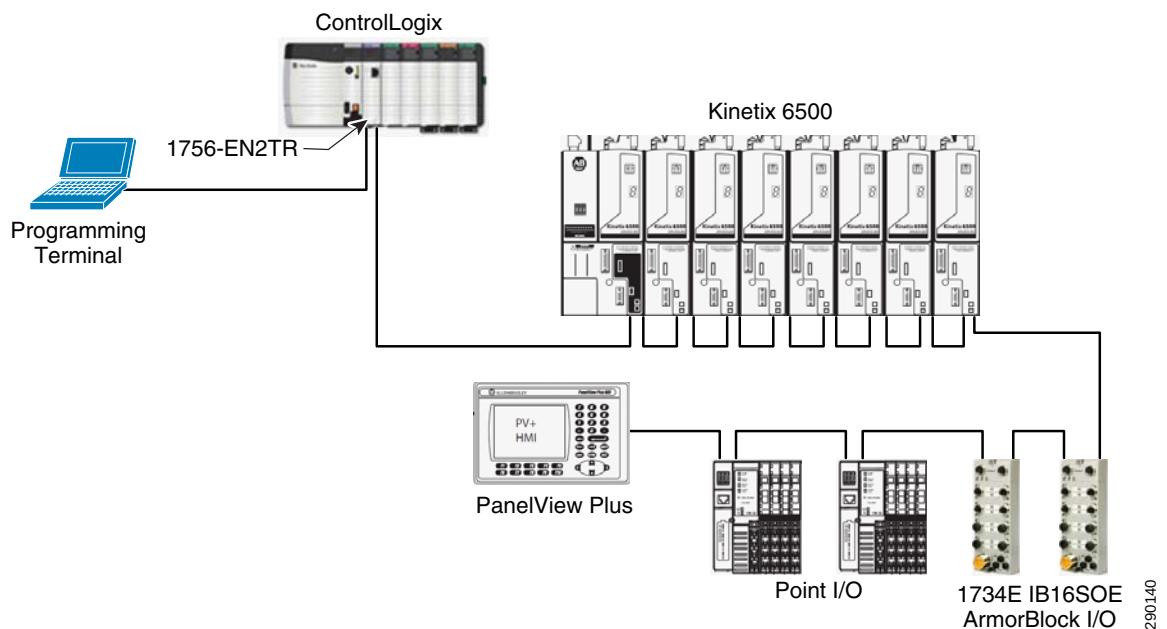
Figure 8-12 Linear Reference Architecture Without Switch
