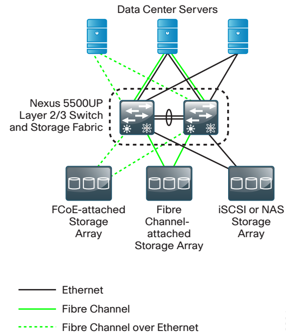
Figure 3 - Cisco SBA data center architecture switch fabric
