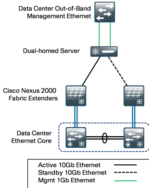
Figure 12 - Cisco UCS C-Series server with separate management interfaces
