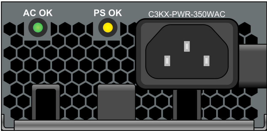
Figure 13 - Power supply option for Cisco Catalyst 3750-X and 3560-X Series switches
