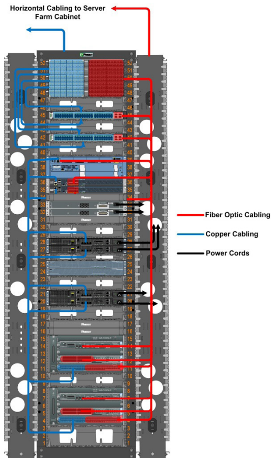
Figure 7 - Cable routing within R1
