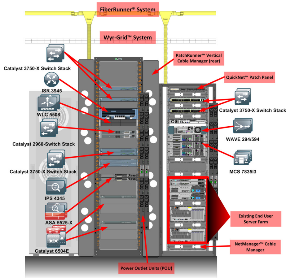
Figure 3 - Rear view of rack elevation of the Cisco SBA foundation module
