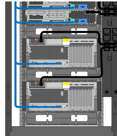
Figure 6 - Close-up view of server farm cable routing
