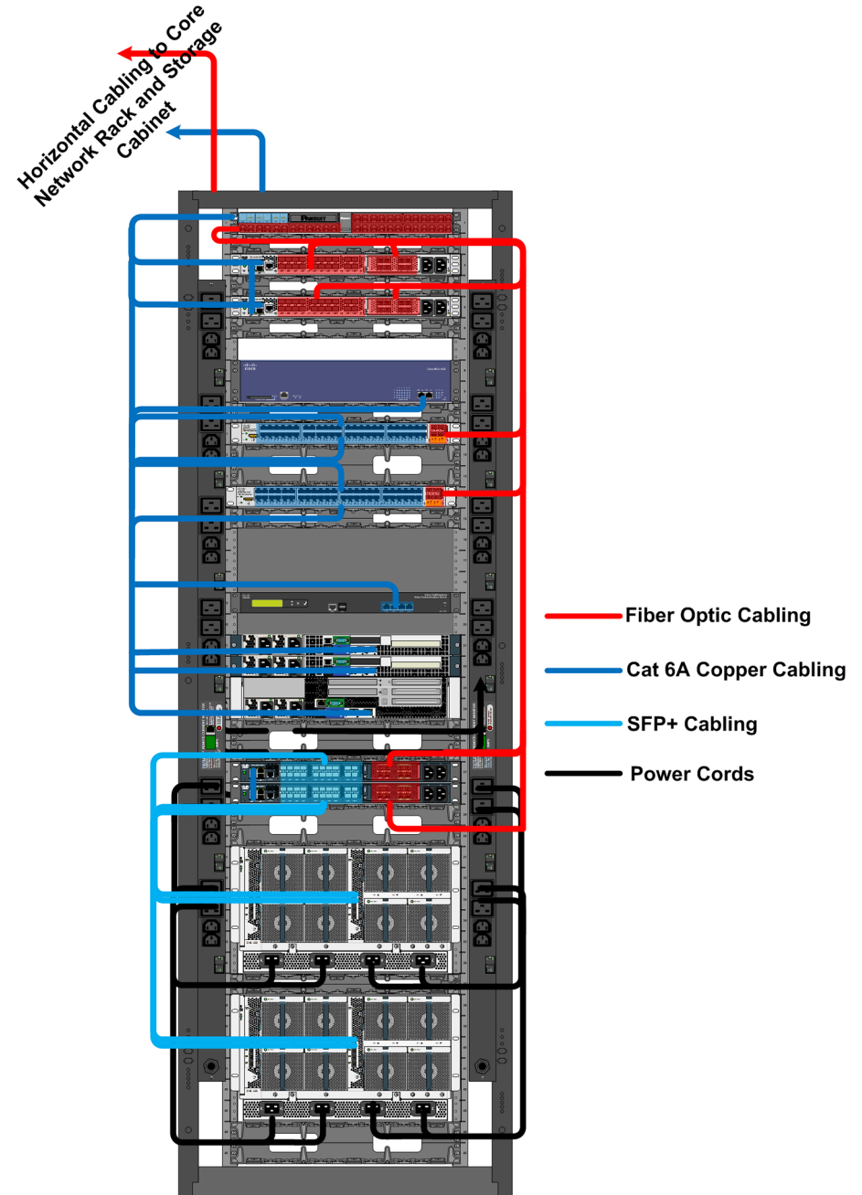
Figure 21 - Cable routing within C2
