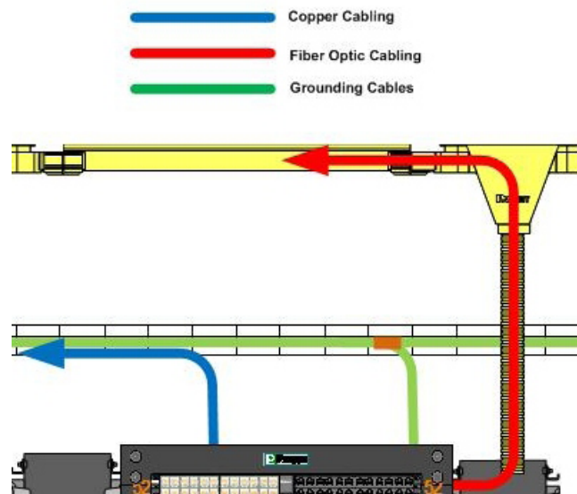
Figure 9 - Close-up view of pathways and cabling over R1
