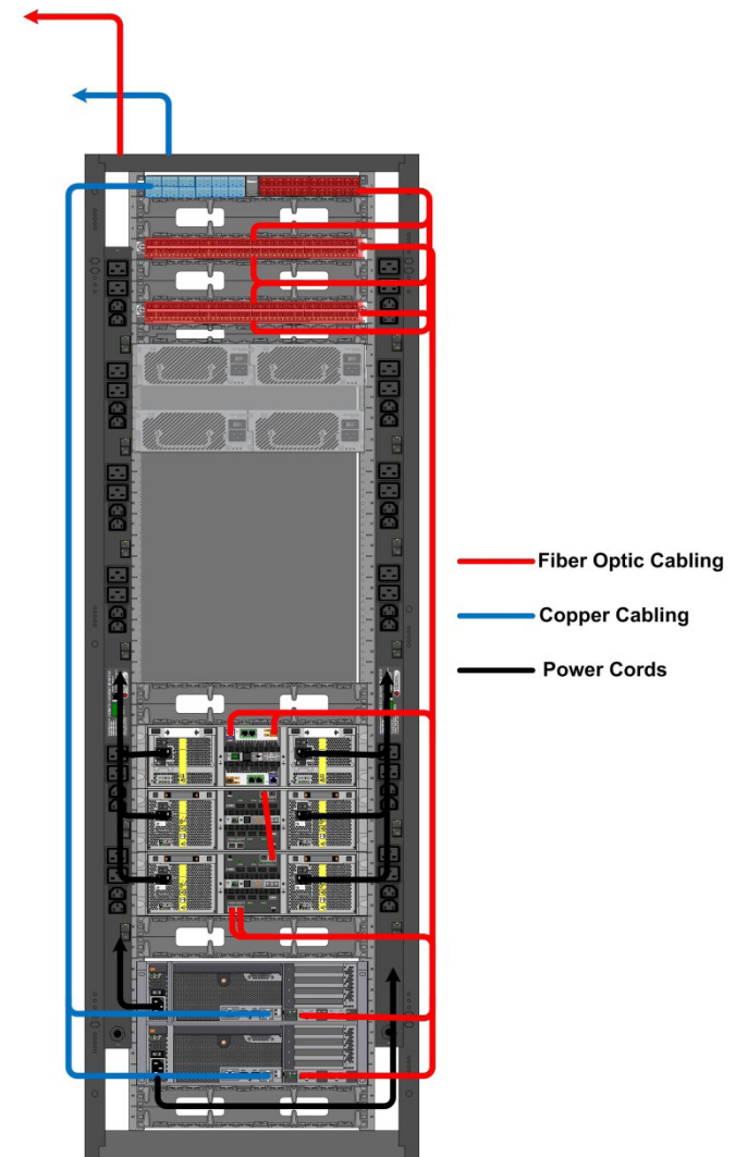
Figure 19 - Cable routing within C3
