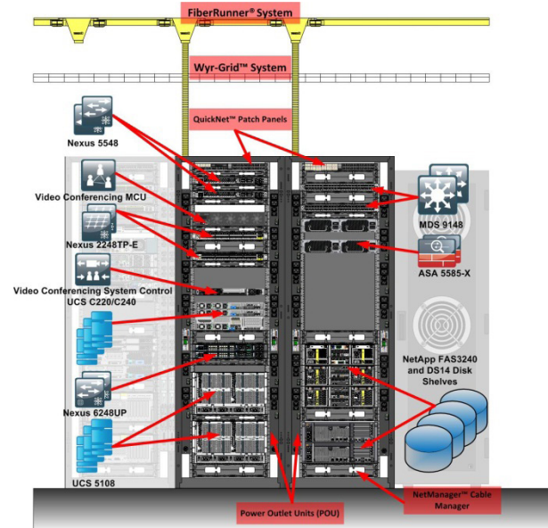
Figure 18 - Rear view of rack elevation of the Cisco SBA data center
