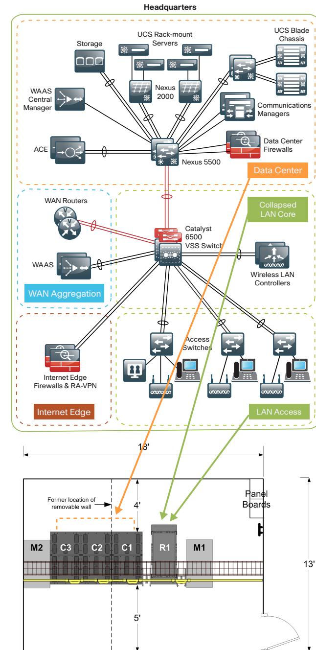
Figure 16 - Top-down view of Cisco SBA data center mapped to the logical architecture
