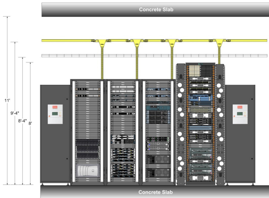
Figure 17 - Front view of rack elevation of the Cisco SBA data center
