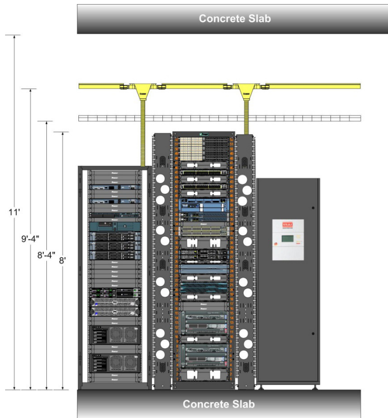
Figure 2 - Front view of rack elevation of the Cisco SBA foundation module
