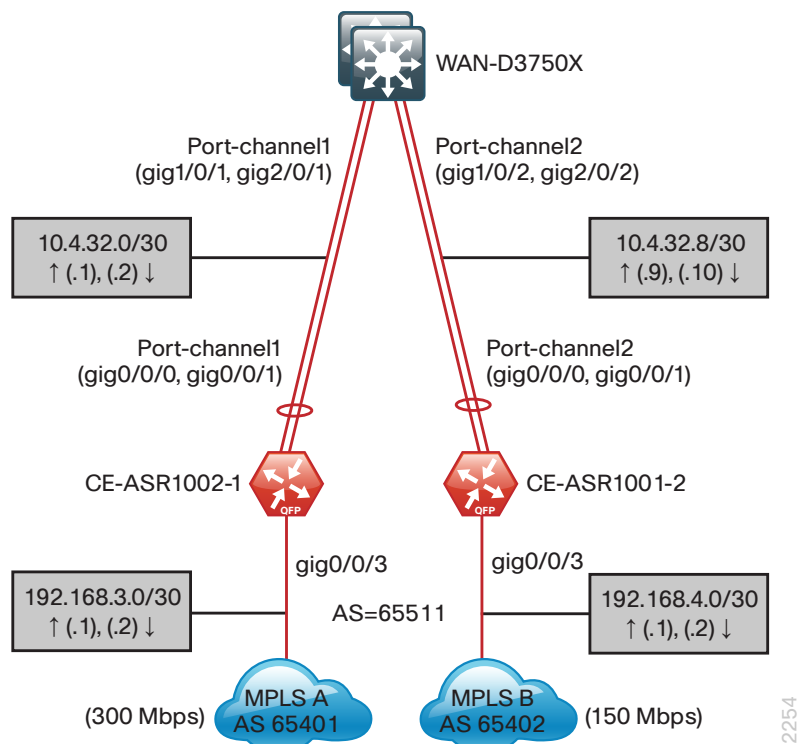
Figure 3 - WAN-aggregation design—Dual MPLS and MPLS Dynamic design models
