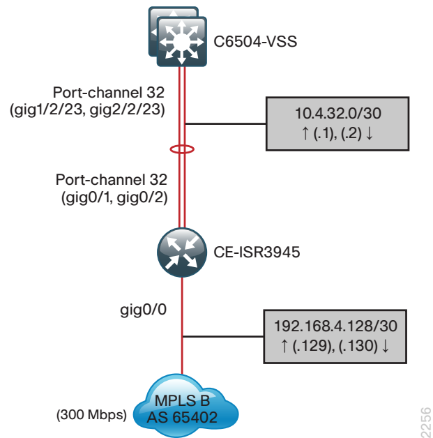
Figure 5 - WAN-aggregation design—MPLS Static
