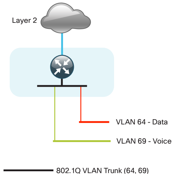
Figure 16 - WAN remote site—Flat Layer 2 LAN (single router)
