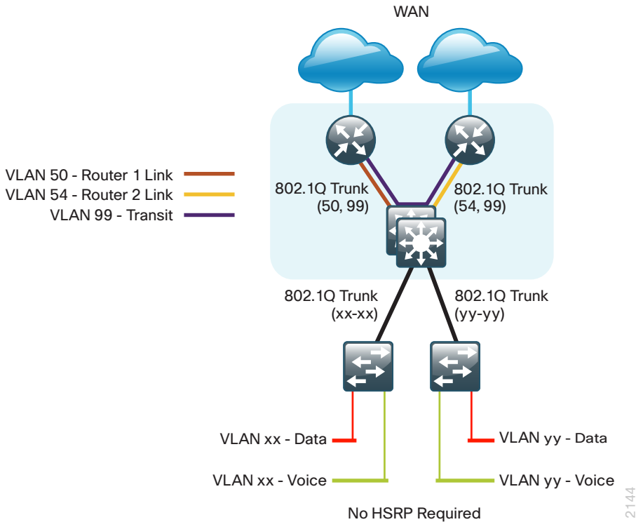
Figure 20 - WAN remote-site—Distribution and access layer (dual router)
