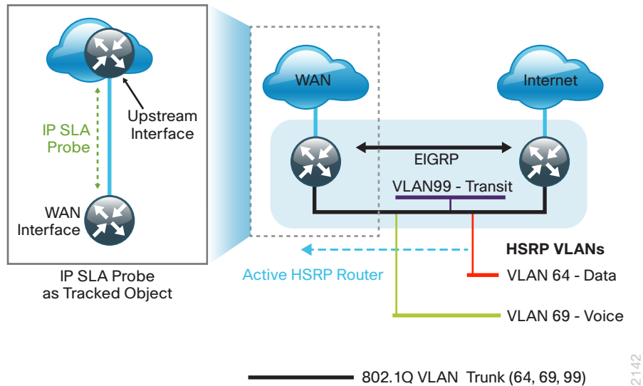
Figure 18 - WAN remote-site—IP SLA probe to verify upstream device reachability
