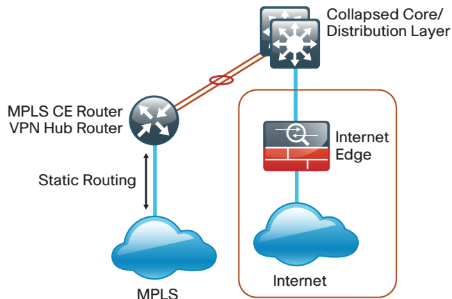
Figure 7 - DMVPN Backup Shared design model
