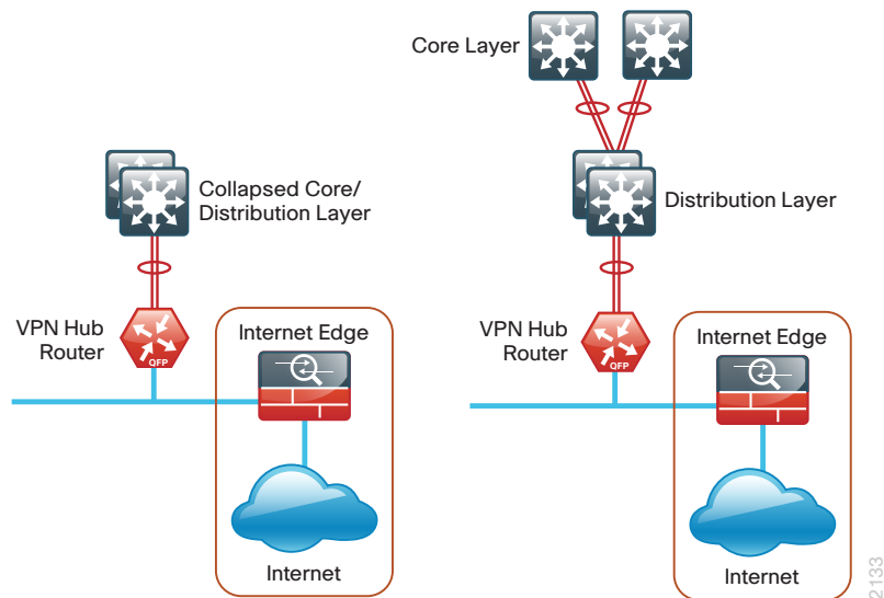
Figure 5 - DMVPN Only design model
