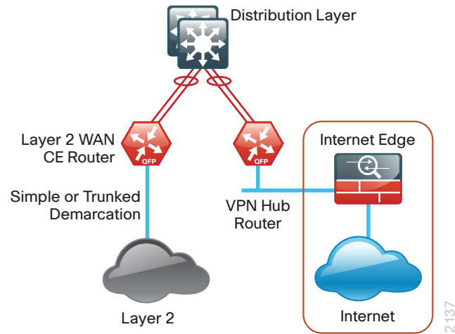
Figure 9 - DMVPN Backup Dedicated design model for Layer 2 WAN primary
