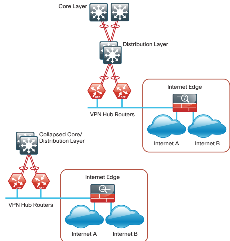
Figure 6 - Dual DMVPN design model
