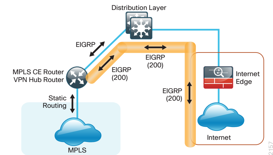
Figure 20 - DMVPN Shared Backup design—Routing details
