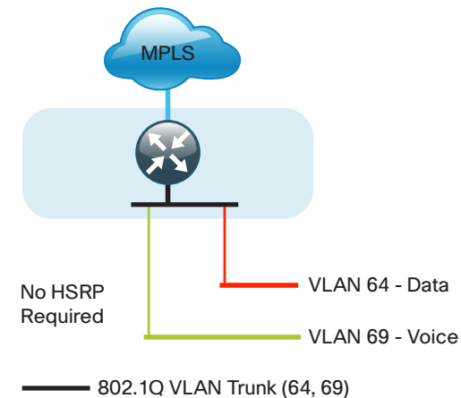
Figure 5 - WAN remote site—Flat Layer 2 LAN (single router)
