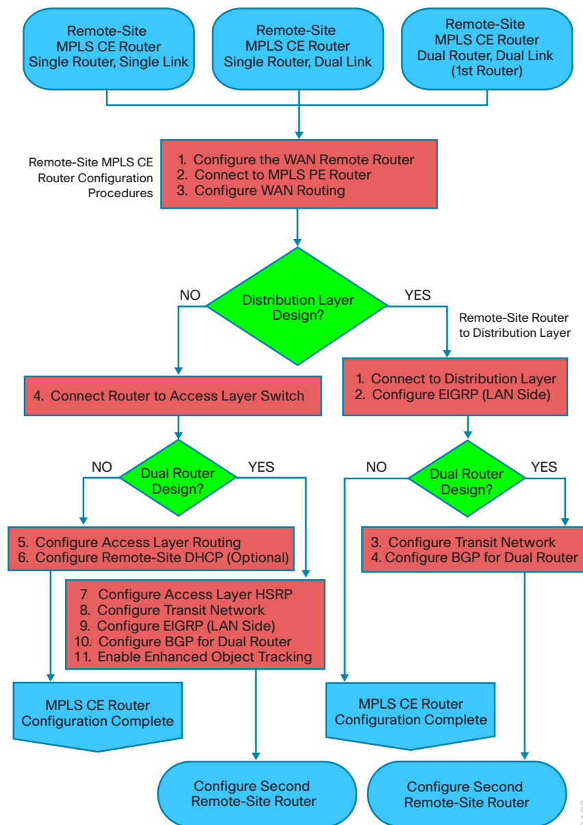
Figure 15 - Remote-site MPLS CE router configuration flowchart
