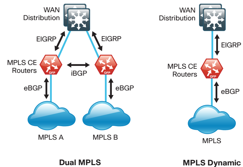
Figure 13 - Dual MPLS and MPLS Dynamic designs—MPLS CE routing detail
