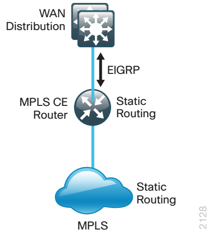
Figure 14 - MPLS Static Design—MPLS CE routing detail
