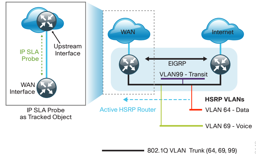
Figure 7 - WAN remote-site - IP SLA probe to verify upstream device reachability
