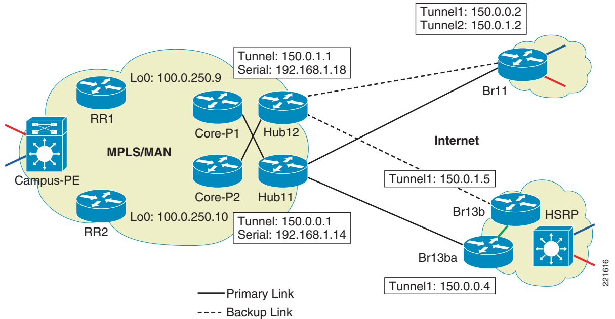
Figure 6-2 2547oDMVPN Redundancy
