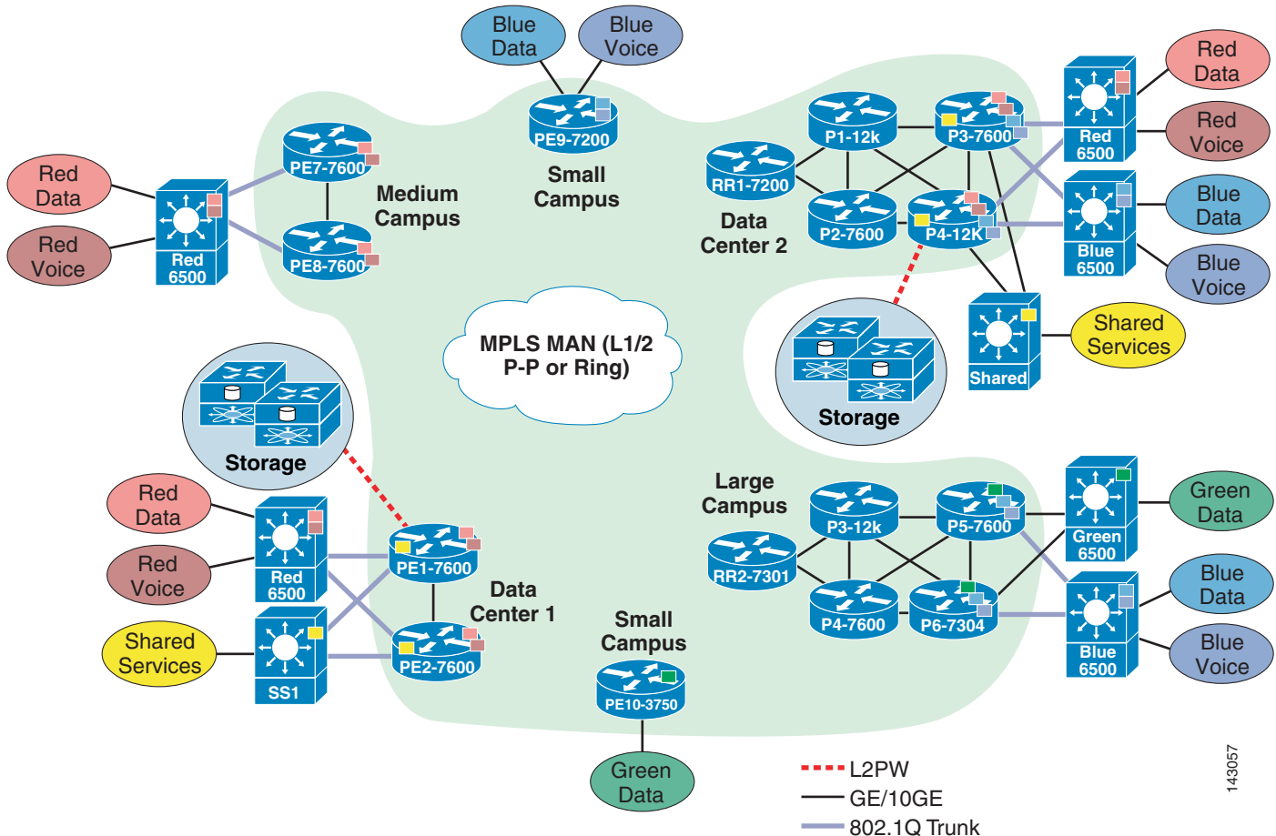
Figure 1-1 Typical Self-Managed MPLS MAN Deployment
