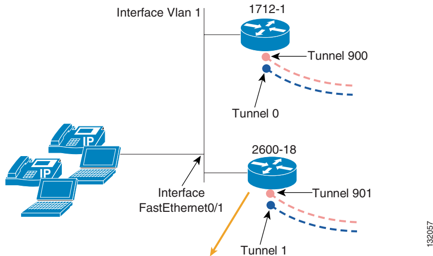
Figure 9-11 Frame Relay/Broadband—CEF/NetFlow Verification
