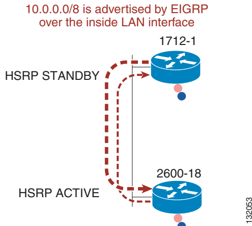
Figure 9-7 Frame Relay/Broadband—10.0.0.0/8 Advertisement
