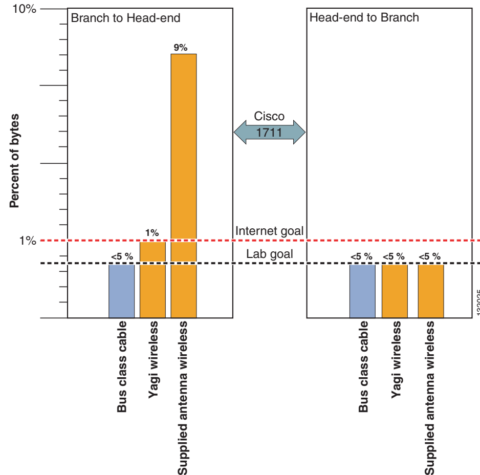
Figure 7-4 Voice Loss
