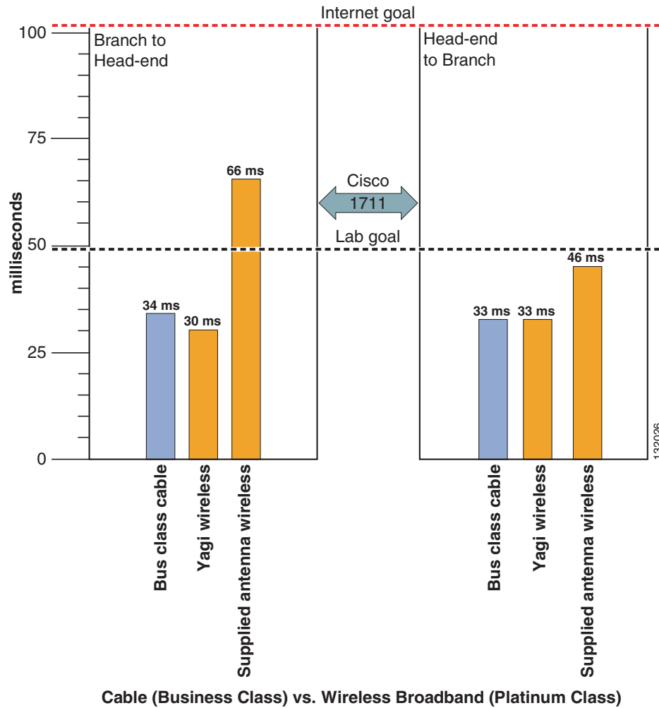
Figure 7-5 Latency
