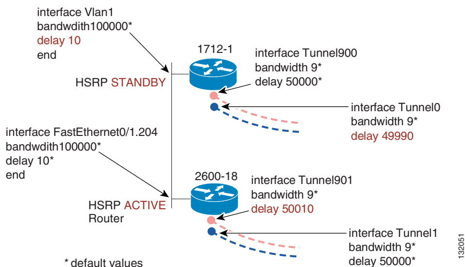
Figure 9-5 Frame Relay/Broadband-Delay/Bandwidth Values
