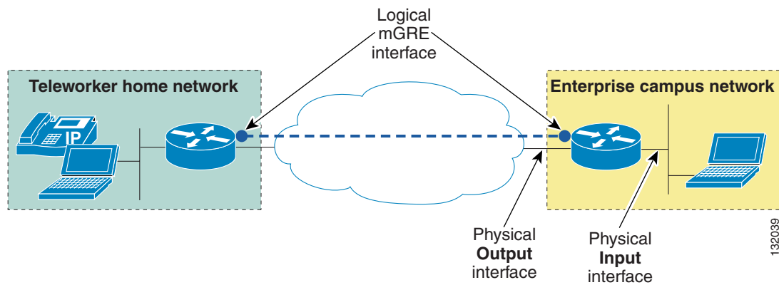
Figure 8-8 Fragmentation Illustration
