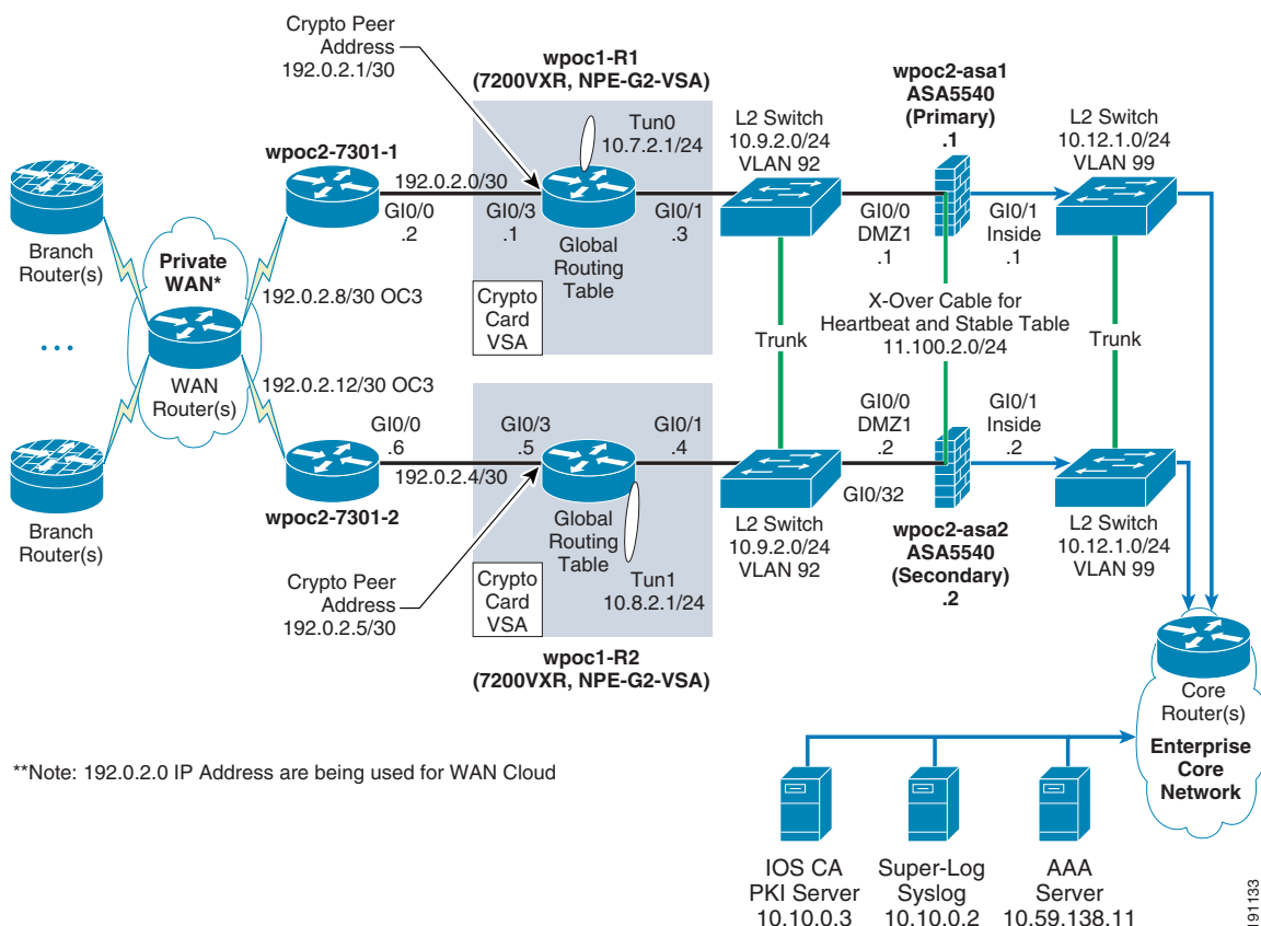
Figure 22 Profile 1 (OC3) Multi-Thread in One Site (Three-Tier Solution)
