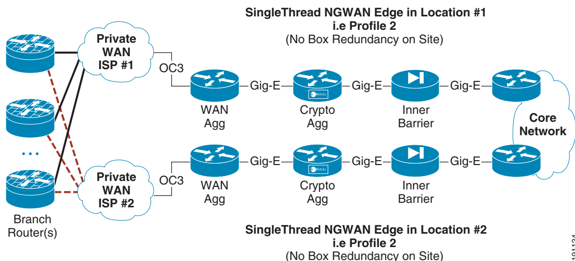
Figure 17 Multi-Site Single-Threaded OC3 Solution
