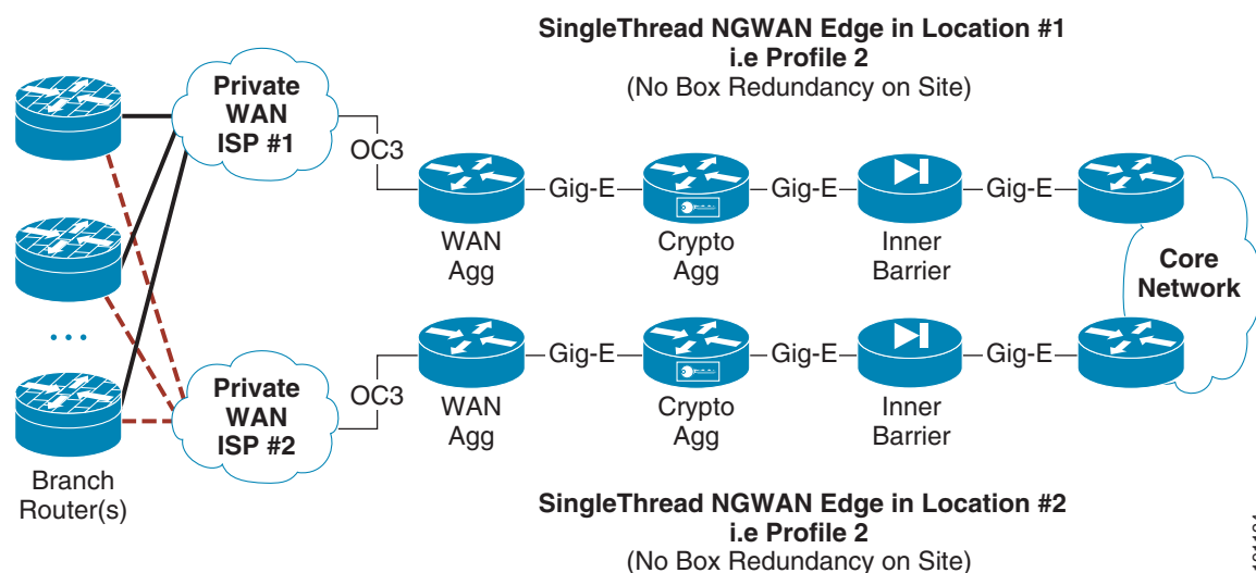
Figure 10 Multiple Single-Threaded Site Locations Redundancy (Profile 1)
