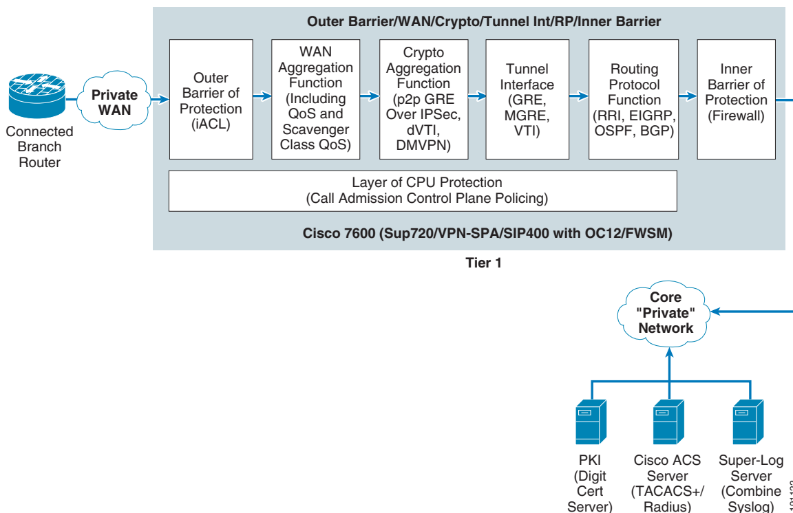
Figure 8 Profile 4 OC12 Architecture (One-Tier Solution)
