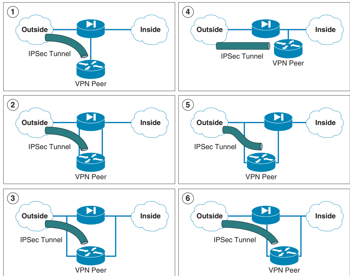
Figure 26 Other VPN/Firewall Topologies
