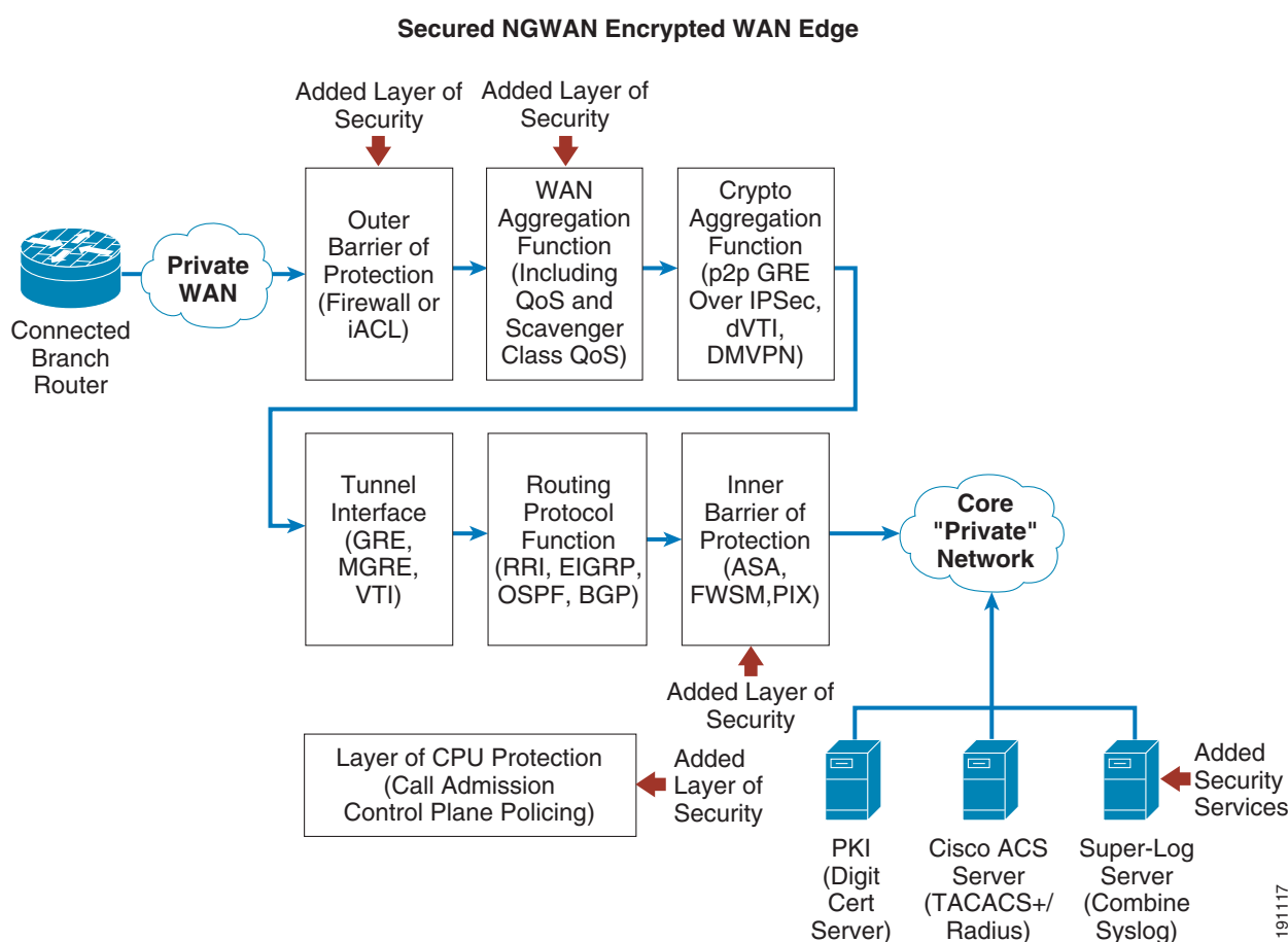
Figure 3 Securing the WAN Edge High-Level Architecture Additional Components
