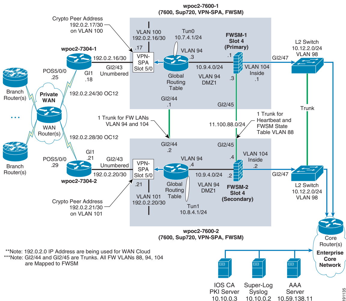
Figure 24 Profile 3 (OC12) Multi-Thread in One Site (Two-Tier Solution)
