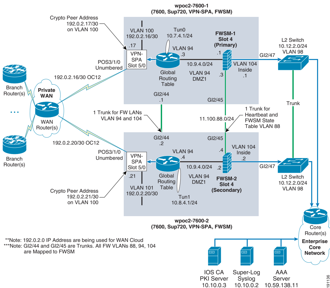
Figure 25 Profile 4 (OC12) Multi-Thread in One Site (One-Tier Solution)
