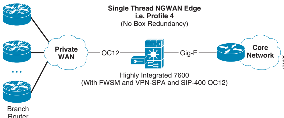
Figure 16 Single-Threaded OC12 Solution
