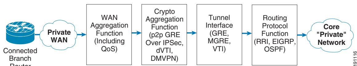
Figure 2 Enterprise WAN and MAN High-Level Architecture Basic Components
