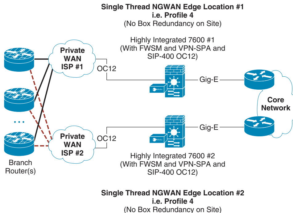
Figure 18 Multi-Site Single-Threaded OC12 Solution
