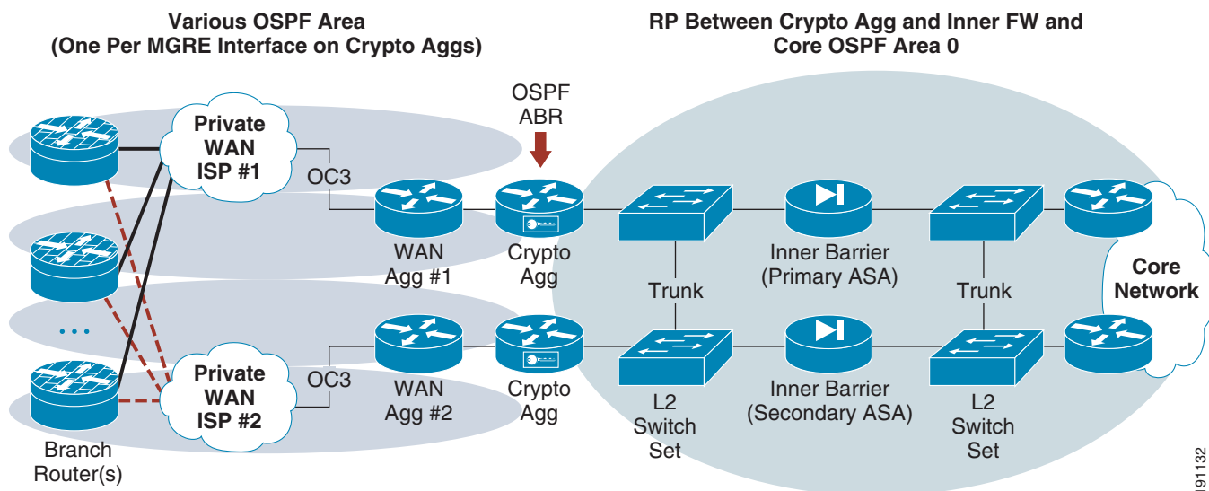
Figure 21 OSPF as only RP
