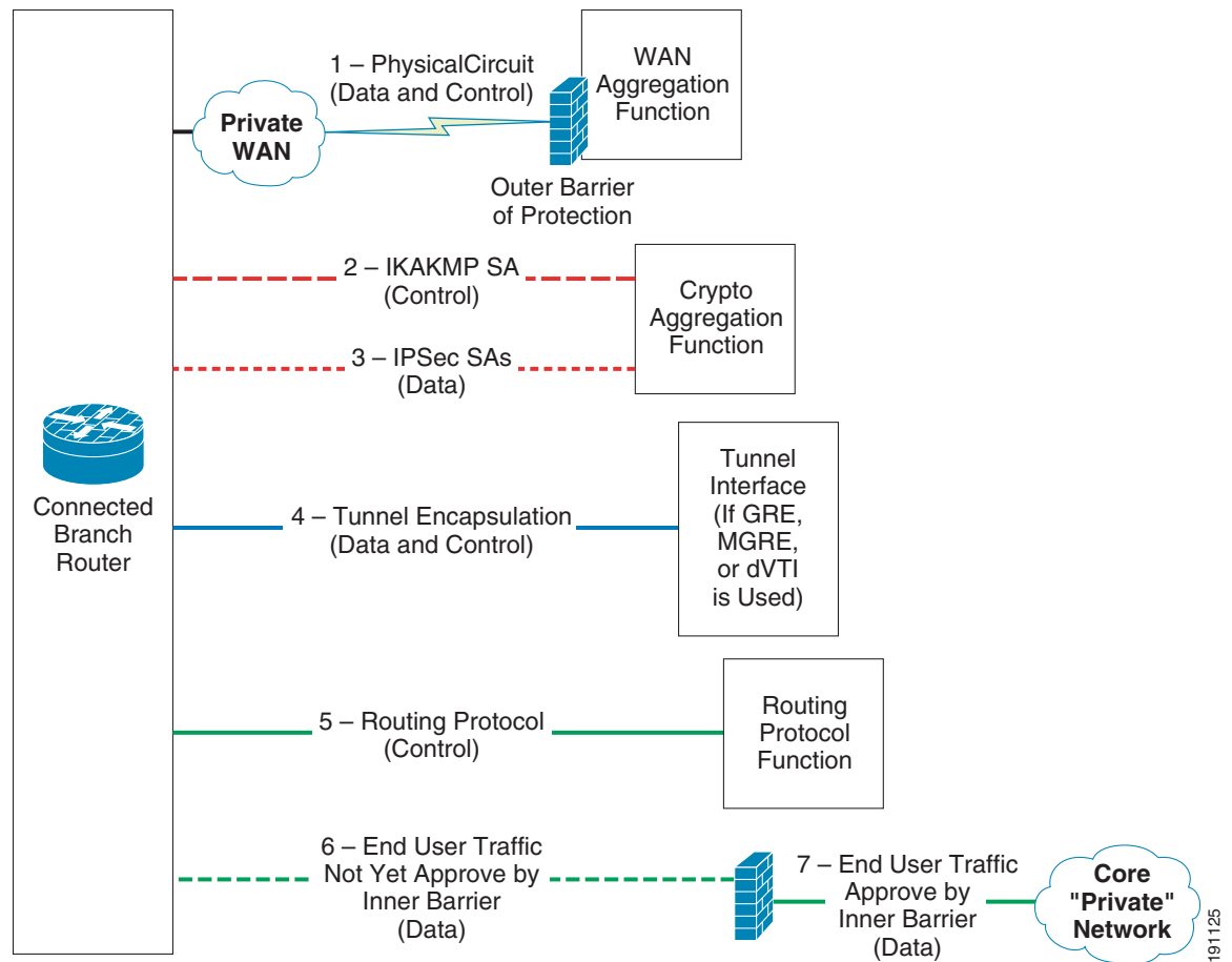
Figure 11 Control Plane versus Data Plane Traffic in NGWAN Edge Architectures
