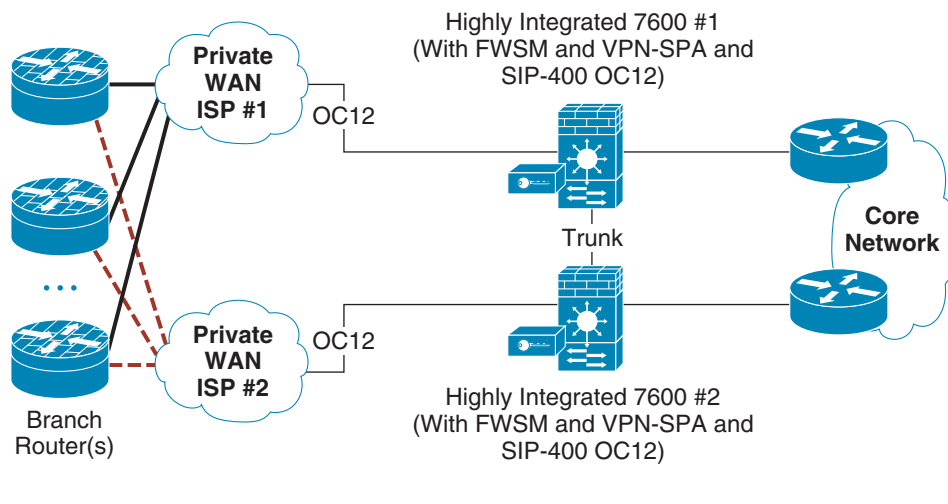
Figure 14 Multi-Threaded Single Site OC12 Solution
