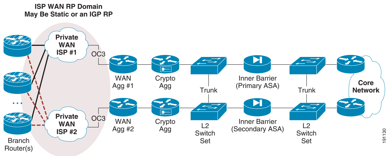
Figure 19 RP used to the ISP
