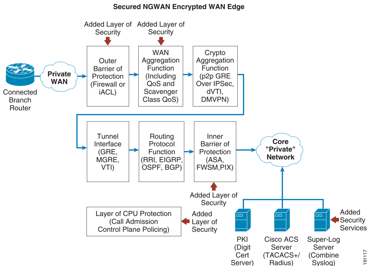
Figure 12 Implementing Security Services and Infrastructure Protections
