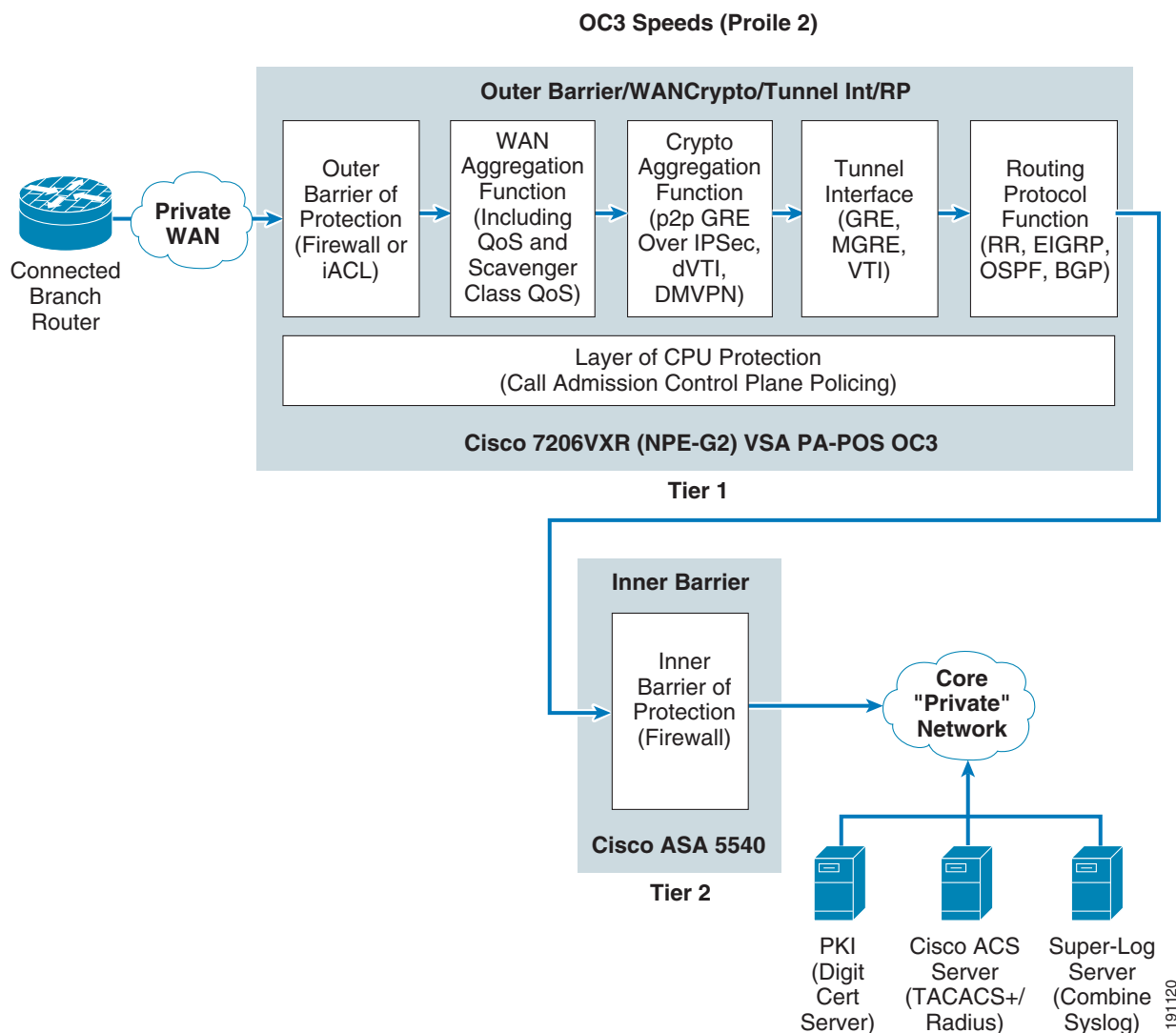
Figure 6 Profile 2 OC3 Architecture (Two-Tier Solution)
