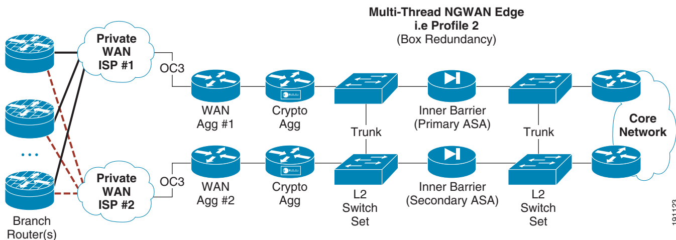
Figure 13 Multi-Threaded Single Site OC3 Solution
