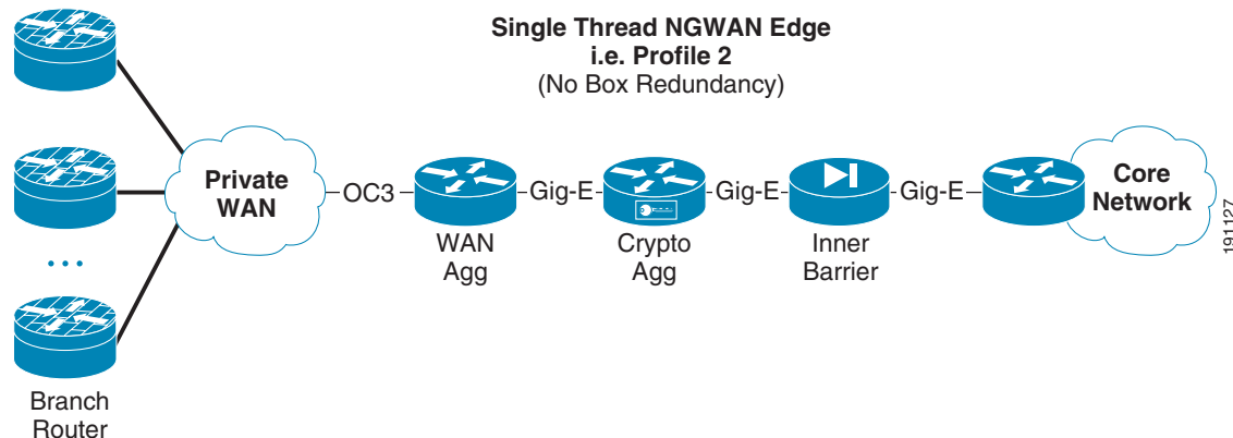
Figure 15 Single-Threaded OC3 Solution
