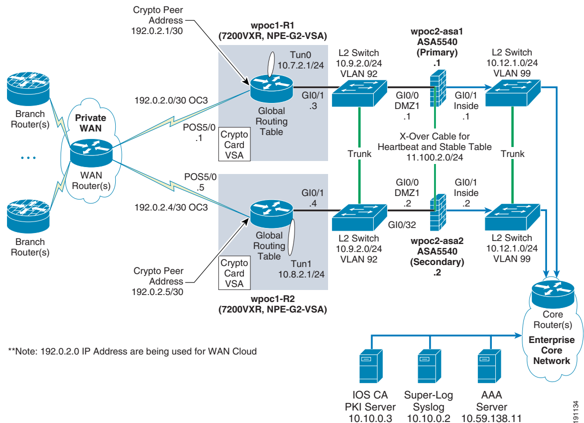
Figure 23 Profile 2 (OC3) Multi-Thread in One Site (Two-Tier Solution)
