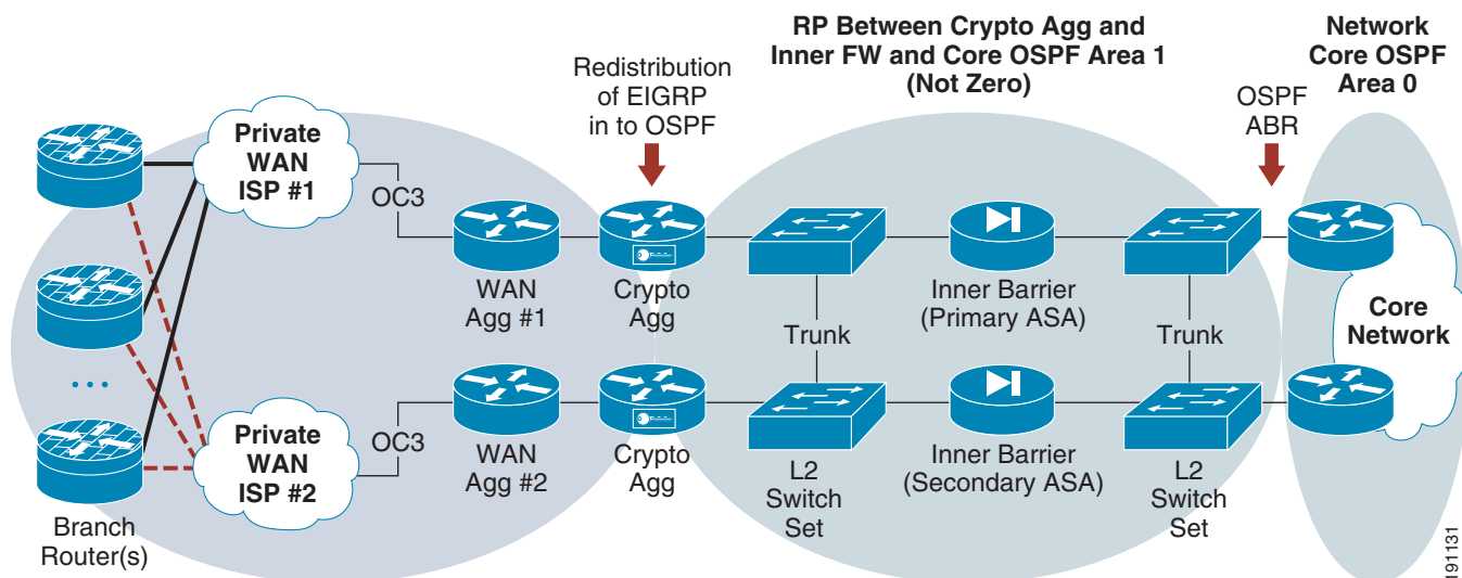
Figure 20 RPs used for the VPN IGP and from the Crypto Aggregation to the Core
