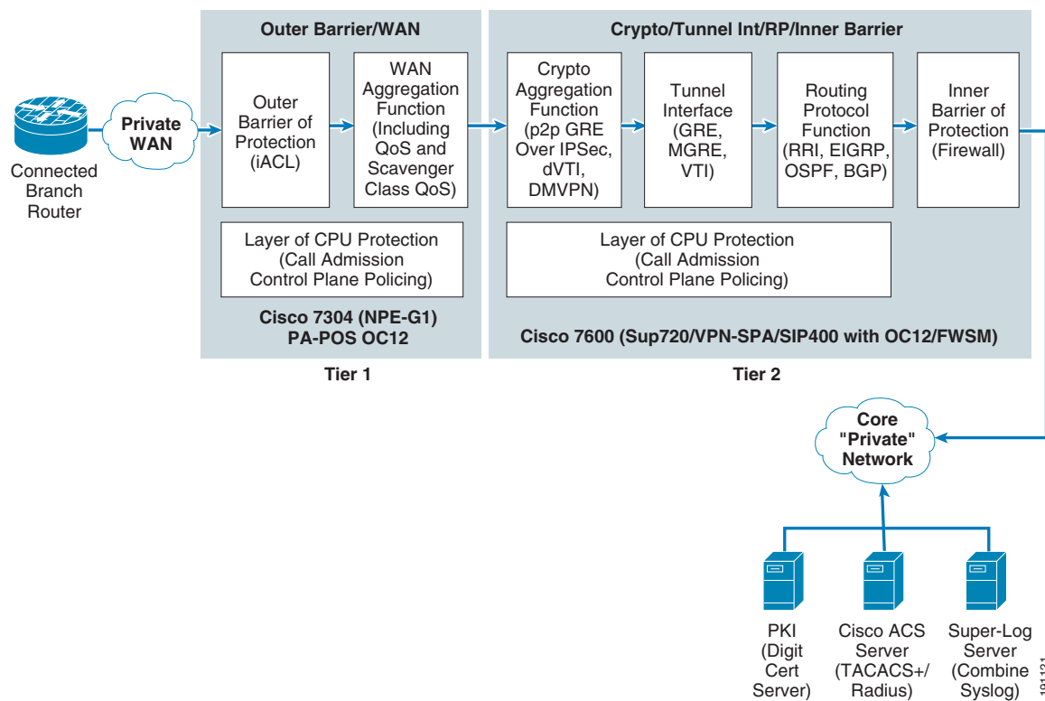
Figure 7 Profile 3 OC12 Architecture (Two-Tier Solution)
