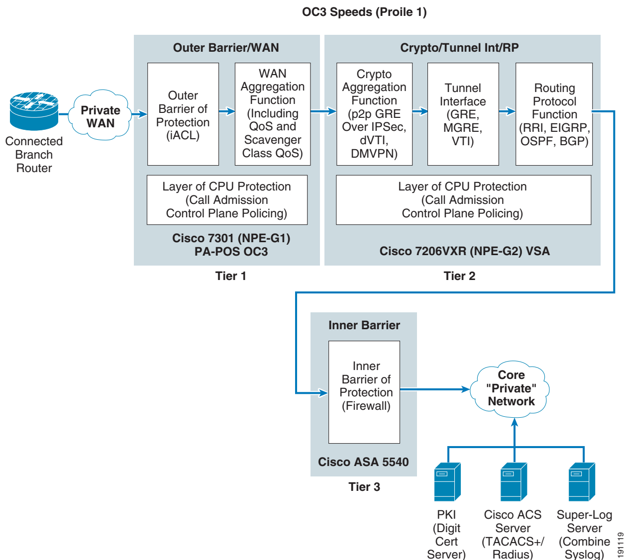
Figure 5 Profile 1 OC3 Architecture (Three-Tier Solution)
