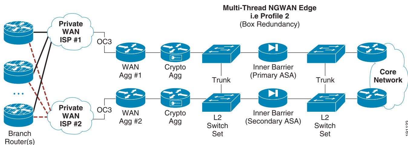
Figure 9 Multi-Threaded System in a Single Location (Profile 1)
